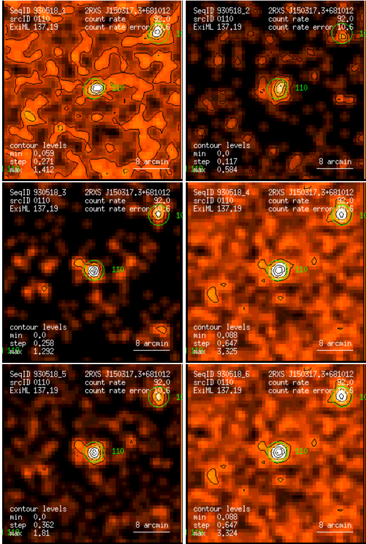
Figure 110: RASS 930518: detection 0110: band rate images, Gaussian filter: (1) PSPC channels 11 – 41, (2) 52 – 90, (3) 91 – 201, (4) 11 – 235, (5) 52 – 201, (6) 11 – 201. Broad band rates in counts/ks. Band rate contour levels in counts/ks/arcmin 2 .
