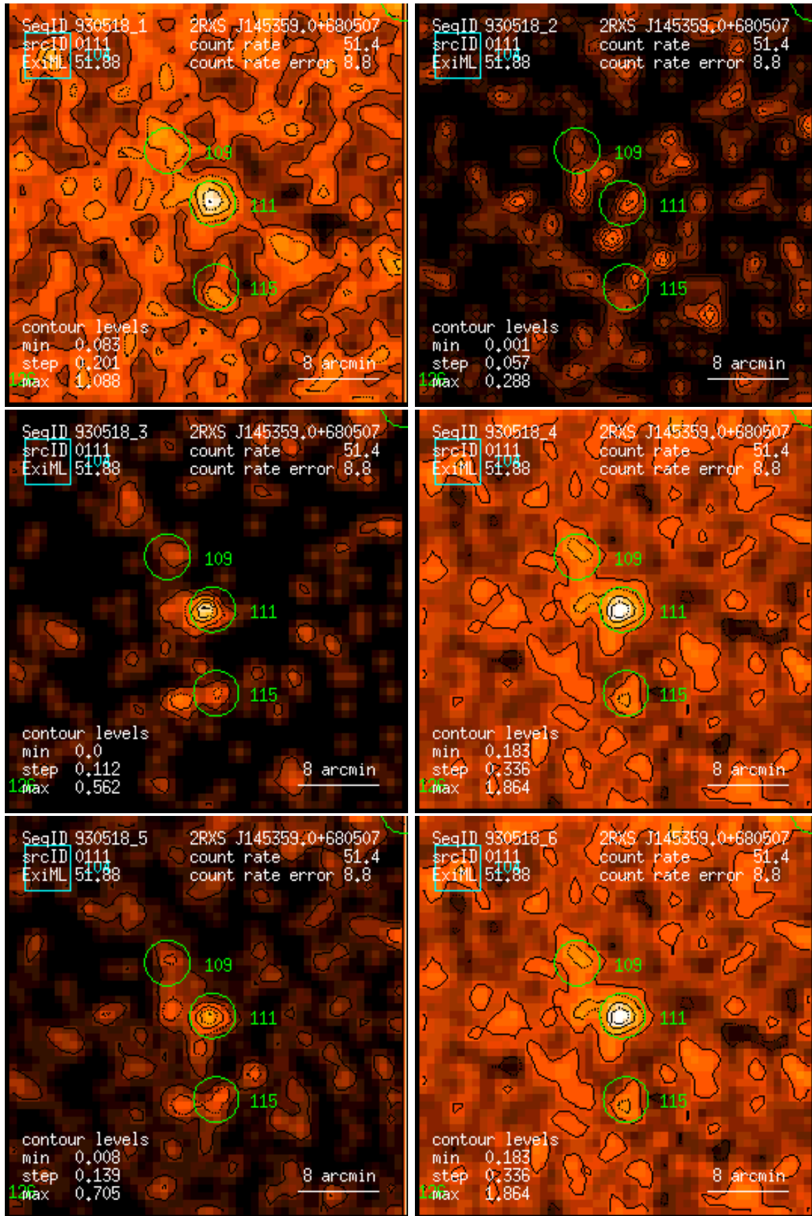
Figure 111: RASS 930518: detection 0111: band rate images, Gaussian filter: (1) PSPC channels 11 – 41, (2) 52 – 90, (3) 91 – 201, (4) 11 – 235, (5) 52 – 201, (6) 11 – 201. Broad band rates in counts/ks. Band rate contour levels in counts/ks/arcmin 2 .
