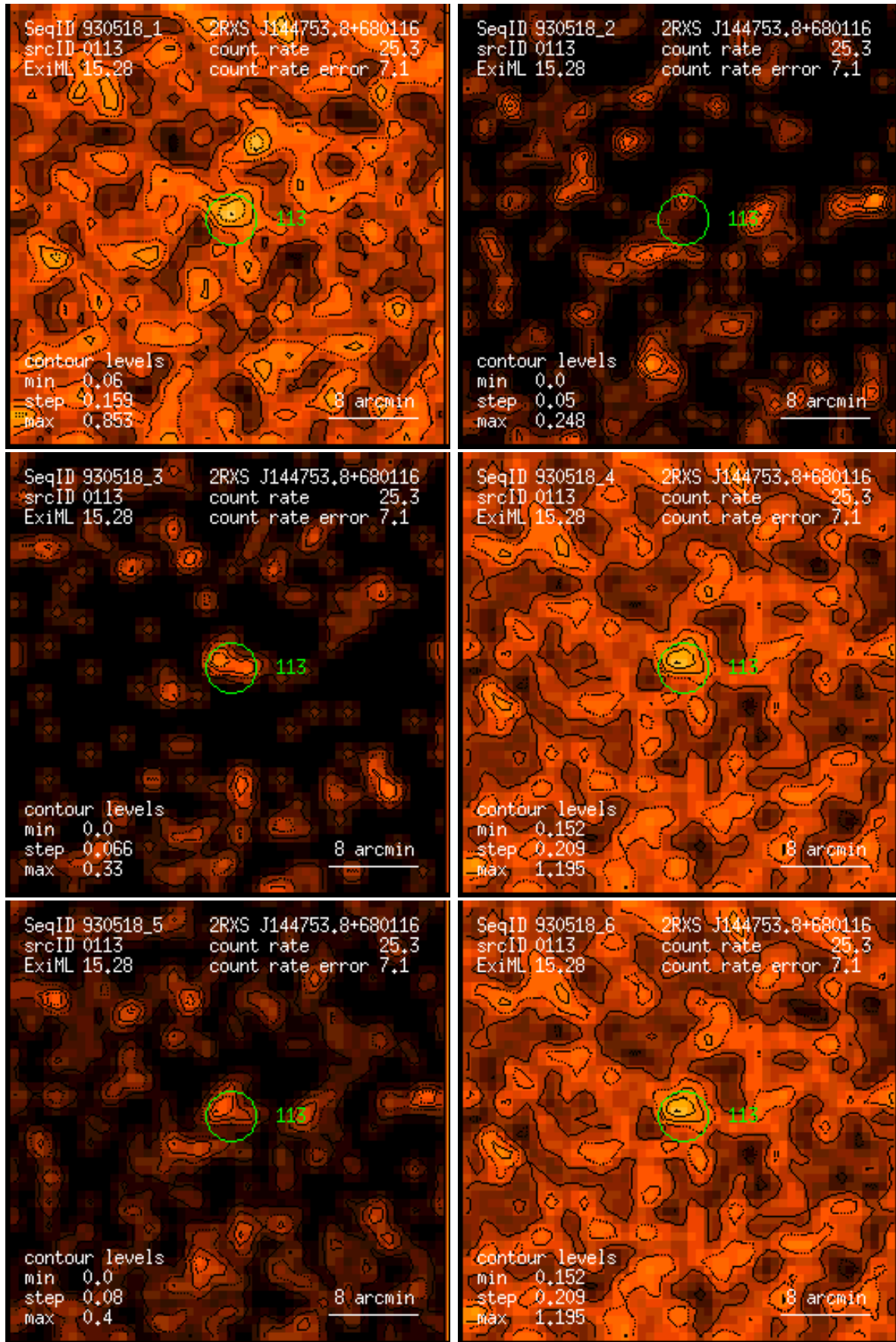
Figure 113: RASS 930518: detection 0113: band rate images, Gaussian filter: (1) PSPC channels 11 – 41, (2) 52 – 90, (3) 91 – 201, (4) 11 – 235, (5) 52 – 201, (6) 11 – 201. Broad band rates in counts/ks. Band rate contour levels in counts/ks/arcmin 2 .
