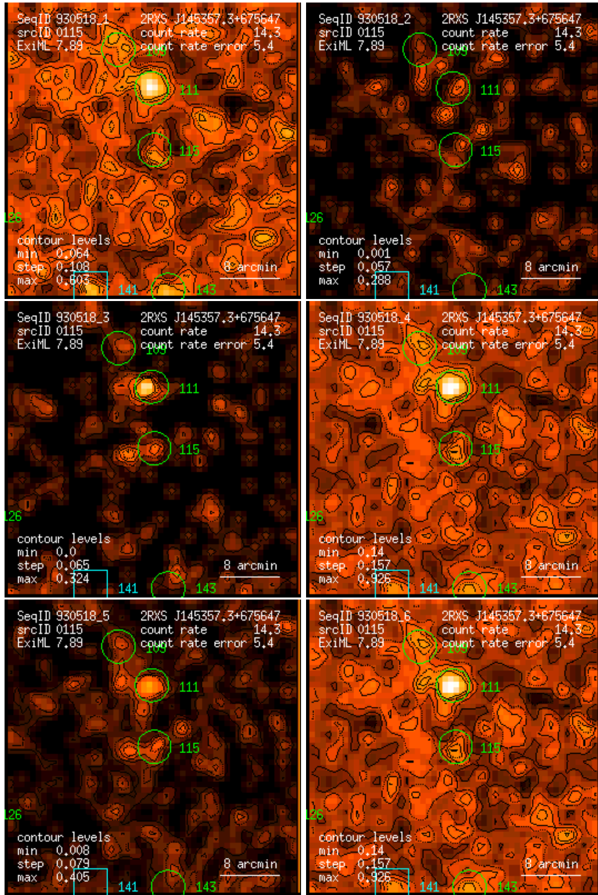
Figure 115: RASS 930518: detection 0115: band rate images, Gaussian filter: (1) PSPC channels 11 – 41, (2) 52 – 90, (3) 91 – 201, (4) 11 – 235, (5) 52 – 201, (6) 11 – 201. Broad band rates in counts/ks. Band rate contour levels in counts/ks/arcmin 2 .
