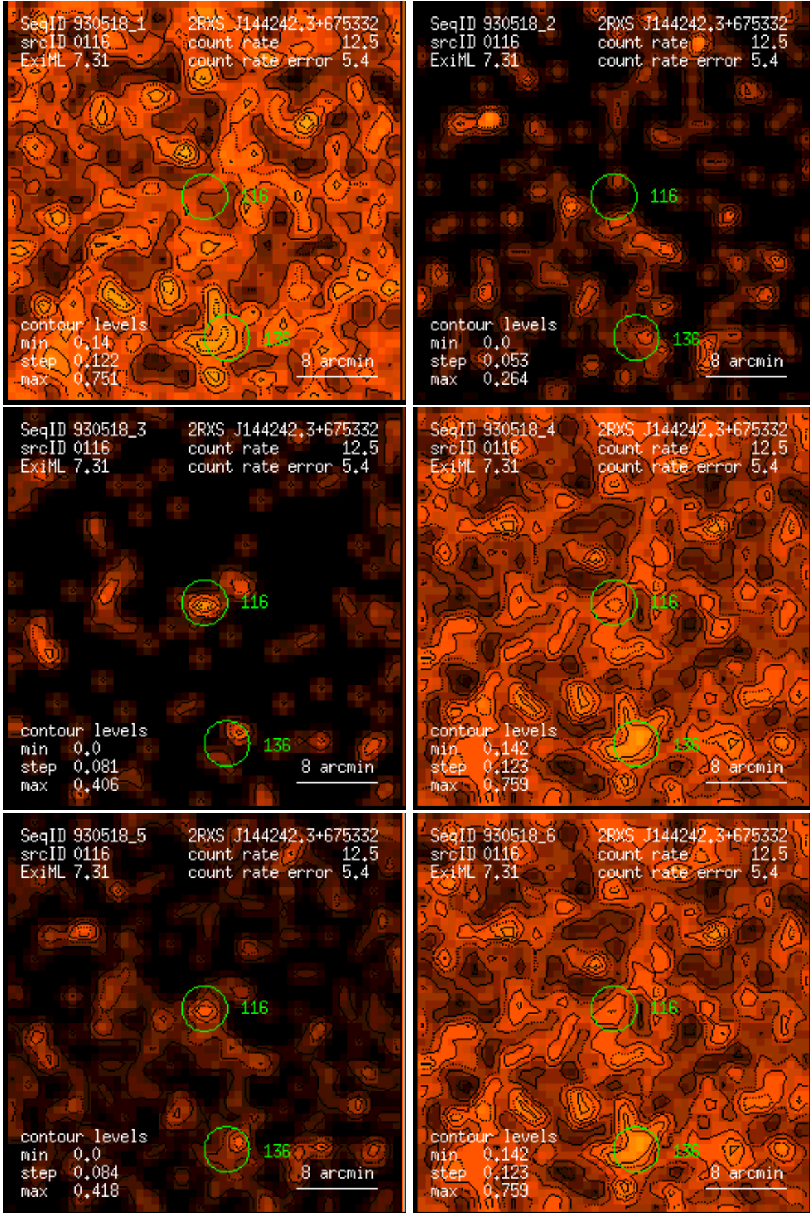
Figure 116: RASS 930518: detection 0116: band rate images, Gaussian filter: (1) PSPC channels 11 – 41, (2) 52 – 90, (3) 91 – 201, (4) 11 – 235, (5) 52 – 201, (6) 11 – 201. Broad band rates in counts/ks. Band rate contour levels in counts/ks/arcmin 2 .
