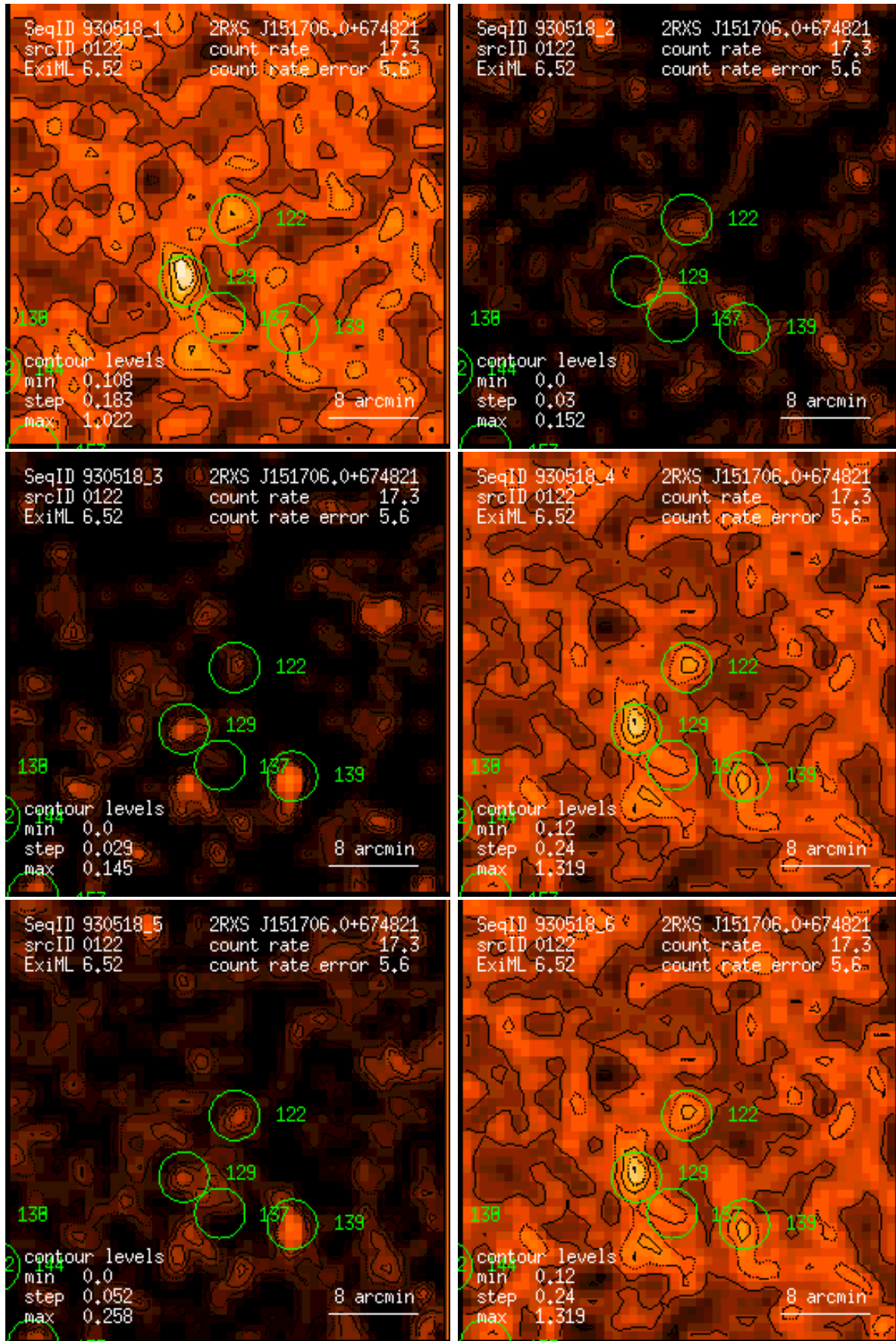
Figure 122: RASS 930518: detection 0122: band rate images, Gaussian filter: (1) PSPC channels 11 – 41, (2) 52 – 90, (3) 91 – 201, (4) 11 – 235, (5) 52 – 201, (6) 11 – 201. Broad band rates in counts/ks. Band rate contour levels in counts/ks/arcmin 2 .
