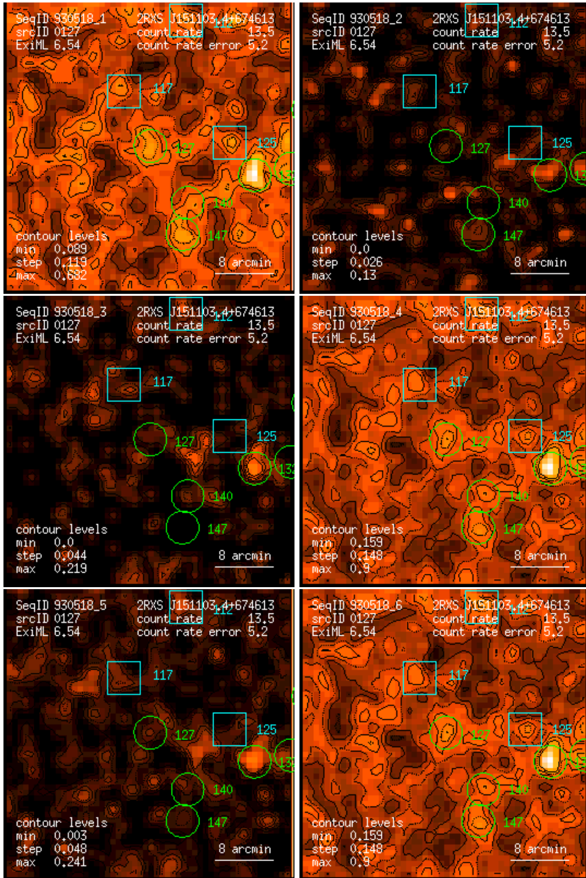
Figure 127: RASS 930518: detection 0127: band rate images, Gaussian filter: (1) PSPC channels 11 – 41, (2) 52 – 90, (3) 91 – 201, (4) 11 – 235, (5) 52 – 201, (6) 11 – 201. Broad band rates in counts/ks. Band rate contour levels in counts/ks/arcmin 2 .
