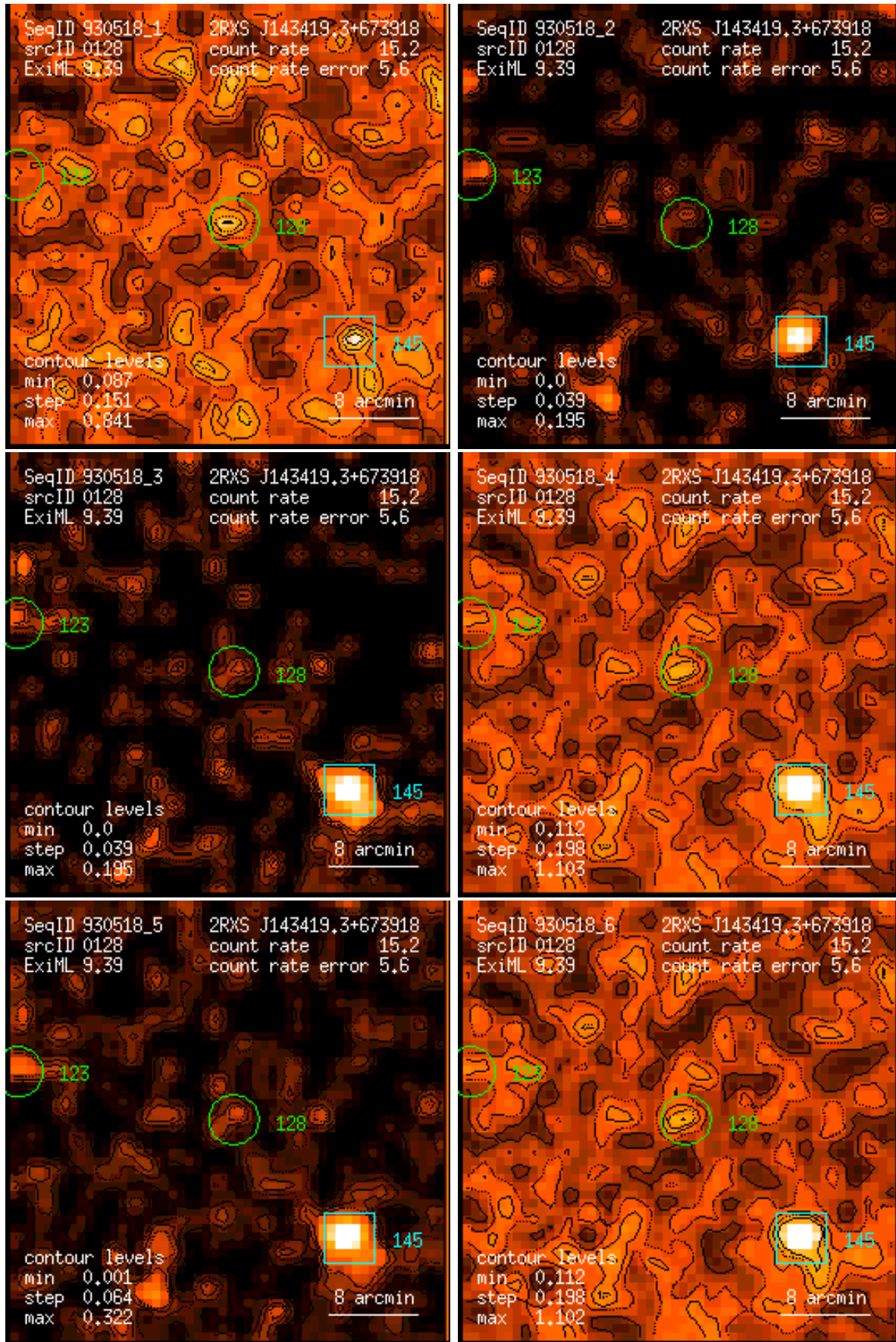
Figure 128: RASS 930518: detection 0128: band rate images, Gaussian filter: (1) PSPC channels 11 – 41, (2) 52 – 90, (3) 91 – 201, (4) 11 – 235, (5) 52 – 201, (6) 11 – 201. Broad band rates in counts/ks. Band rate contour levels in counts/ks/arcmin 2 .
