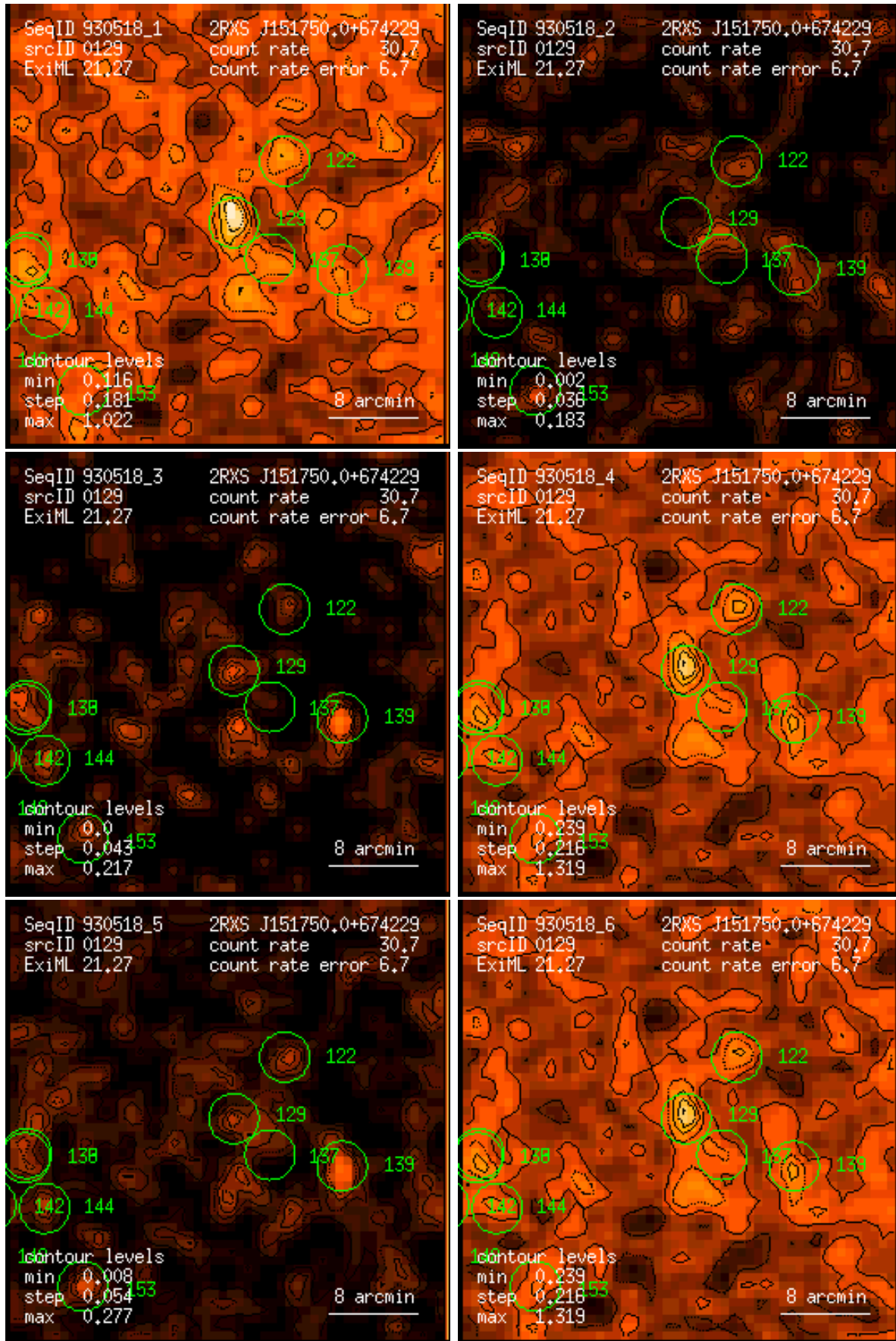
Figure 129: RASS 930518: detection 0129: band rate images, Gaussian filter: (1) PSPC channels 11 – 41, (2) 52 – 90, (3) 91 – 201, (4) 11 – 235, (5) 52 – 201, (6) 11 – 201. Broad band rates in counts/ks. Band rate contour levels in counts/ks/arcmin 2 .
