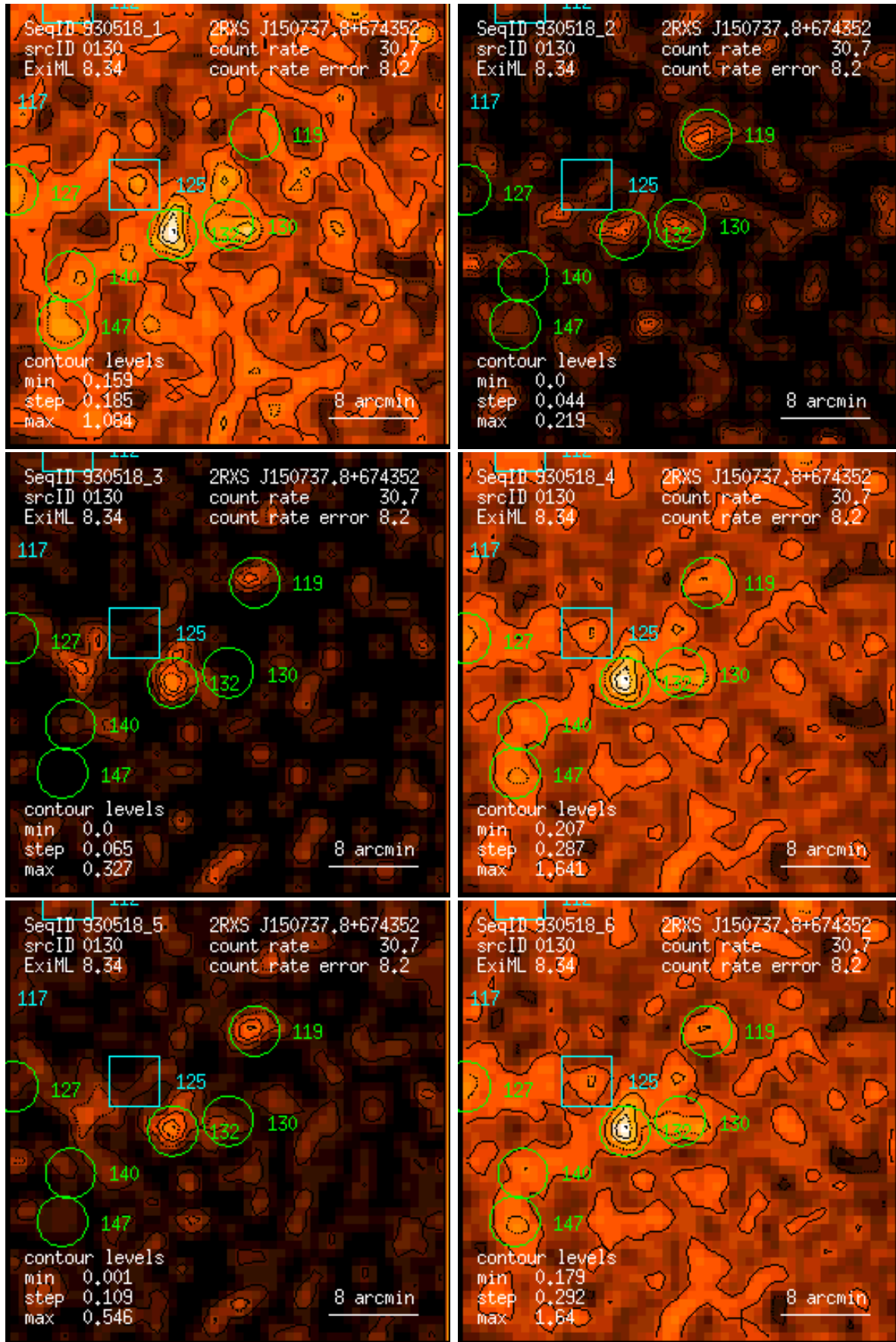
Figure 130: RASS 930518: detection 0130: band rate images, Gaussian filter: (1) PSPC channels 11 – 41, (2) 52 – 90, (3) 91 – 201, (4) 11 – 235, (5) 52 – 201, (6) 11 – 201. Broad band rates in counts/ks. Band rate contour levels in counts/ks/arcmin 2 .
