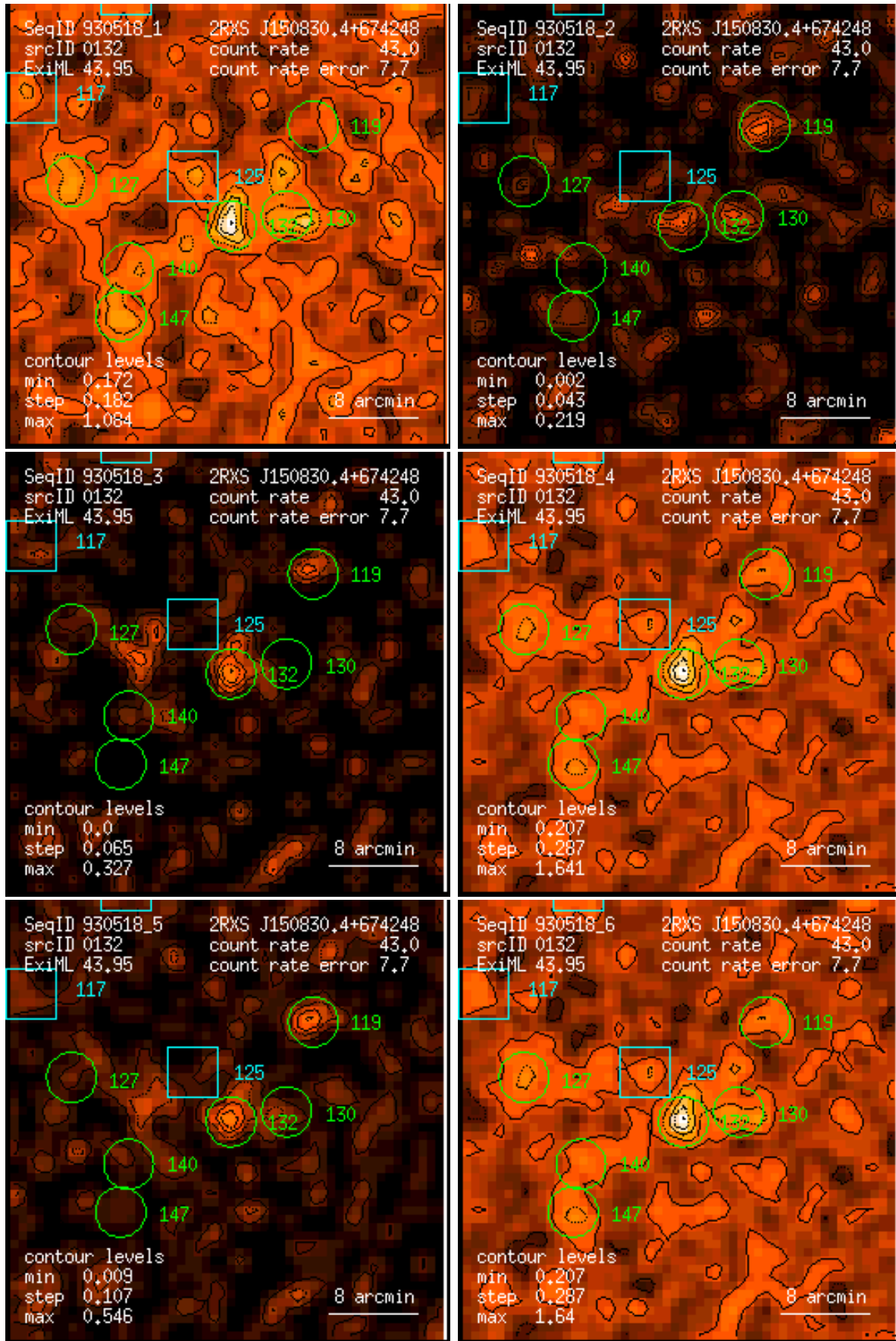
Figure 132: RASS 930518: detection 0132: band rate images, Gaussian filter: (1) PSPC channels 11 – 41, (2) 52 – 90, (3) 91 – 201, (4) 11 – 235, (5) 52 – 201, (6) 11 – 201. Broad band rates in counts/ks. Band rate contour levels in counts/ks/arcmin 2 .
