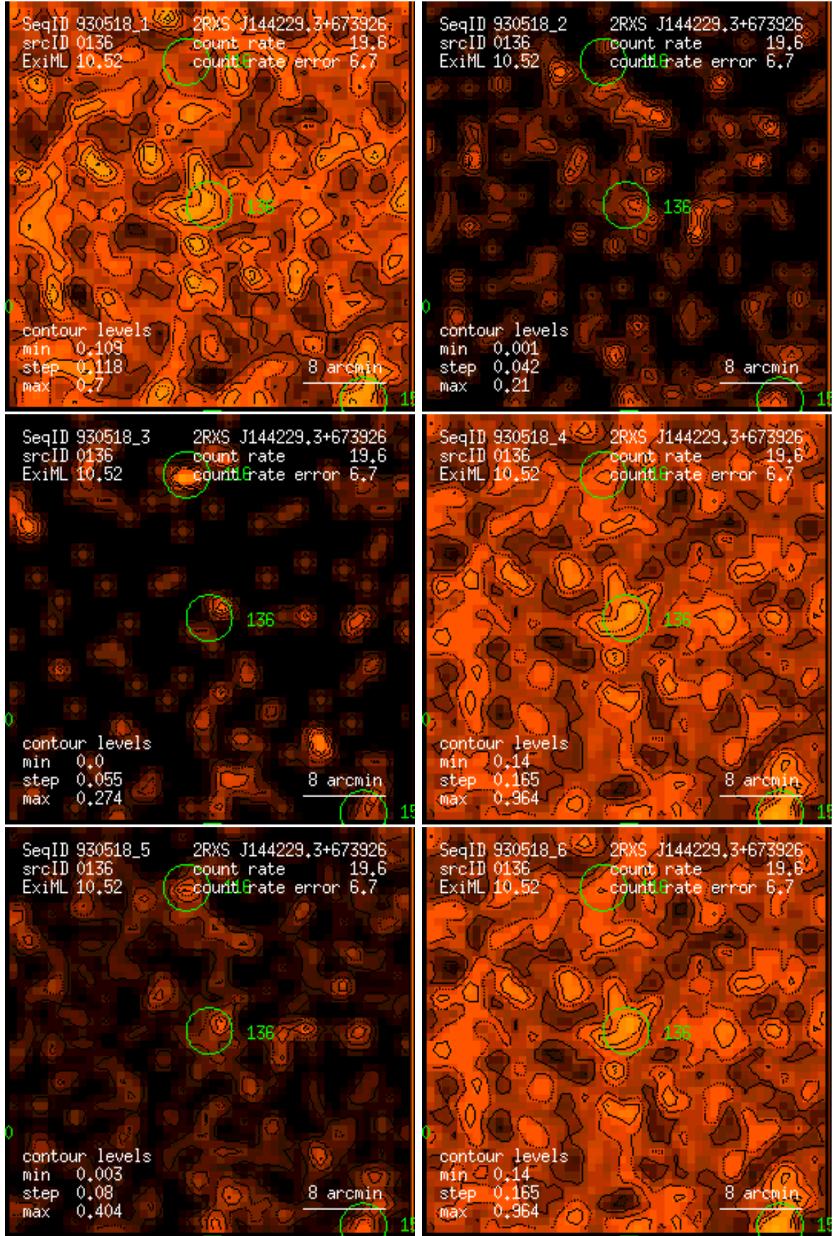
Figure 136: RASS 930518: detection 0136: band rate images, Gaussian filter: (1) PSPC channels 11 – 41, (2) 52 – 90, (3) 91 – 201, (4) 11 – 235, (5) 52 – 201, (6) 11 – 201. Broad band rates in counts/ks. Band rate contour levels in counts/ks/arcmin 2 .
