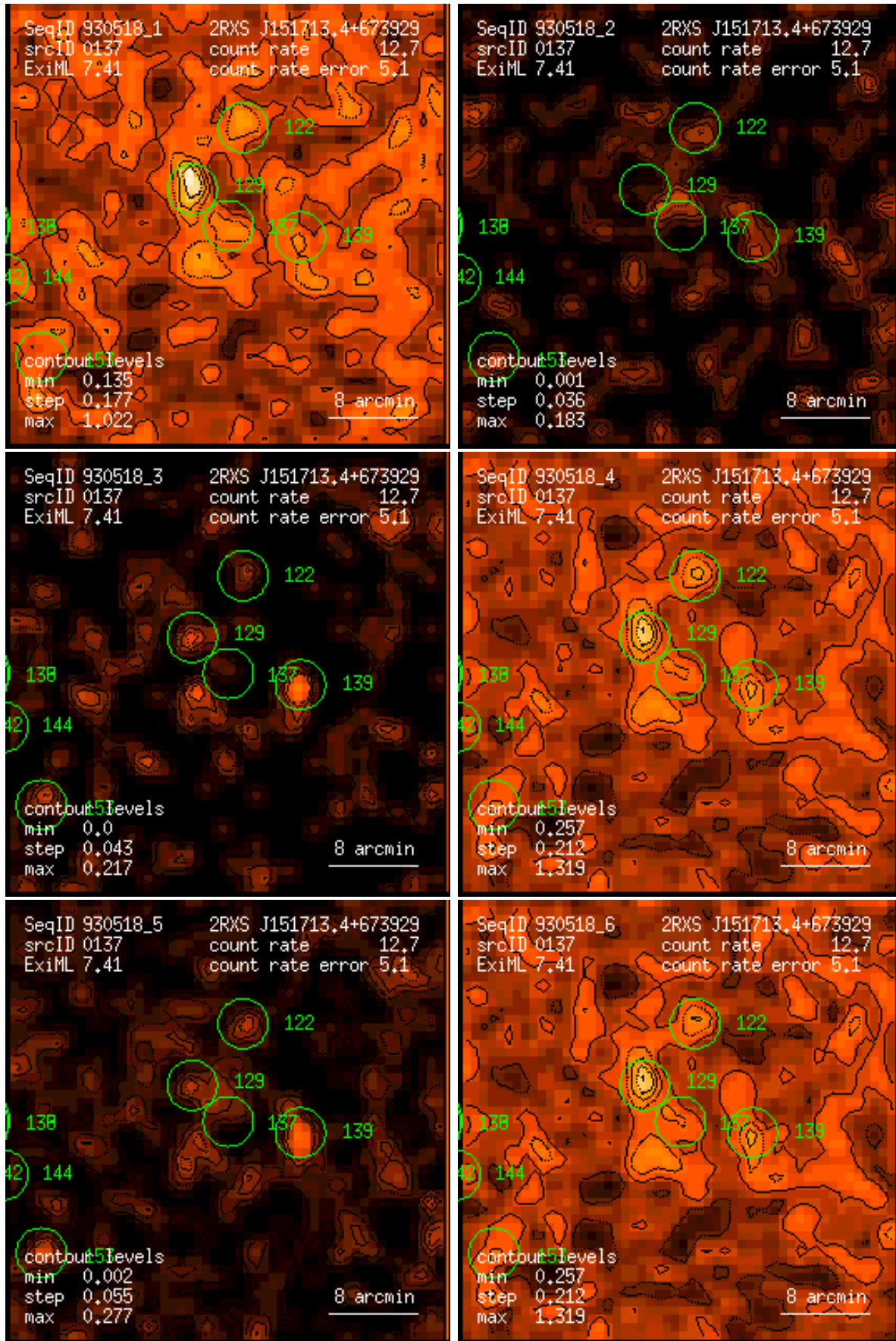
Figure 137: RASS 930518: detection 0137: band rate images, Gaussian filter: (1) PSPC channels 11 – 41, (2) 52 – 90, (3) 91 – 201, (4) 11 – 235, (5) 52 – 201, (6) 11 – 201. Broad band rates in counts/ks. Band rate contour levels in counts/ks/arcmin 2 .
