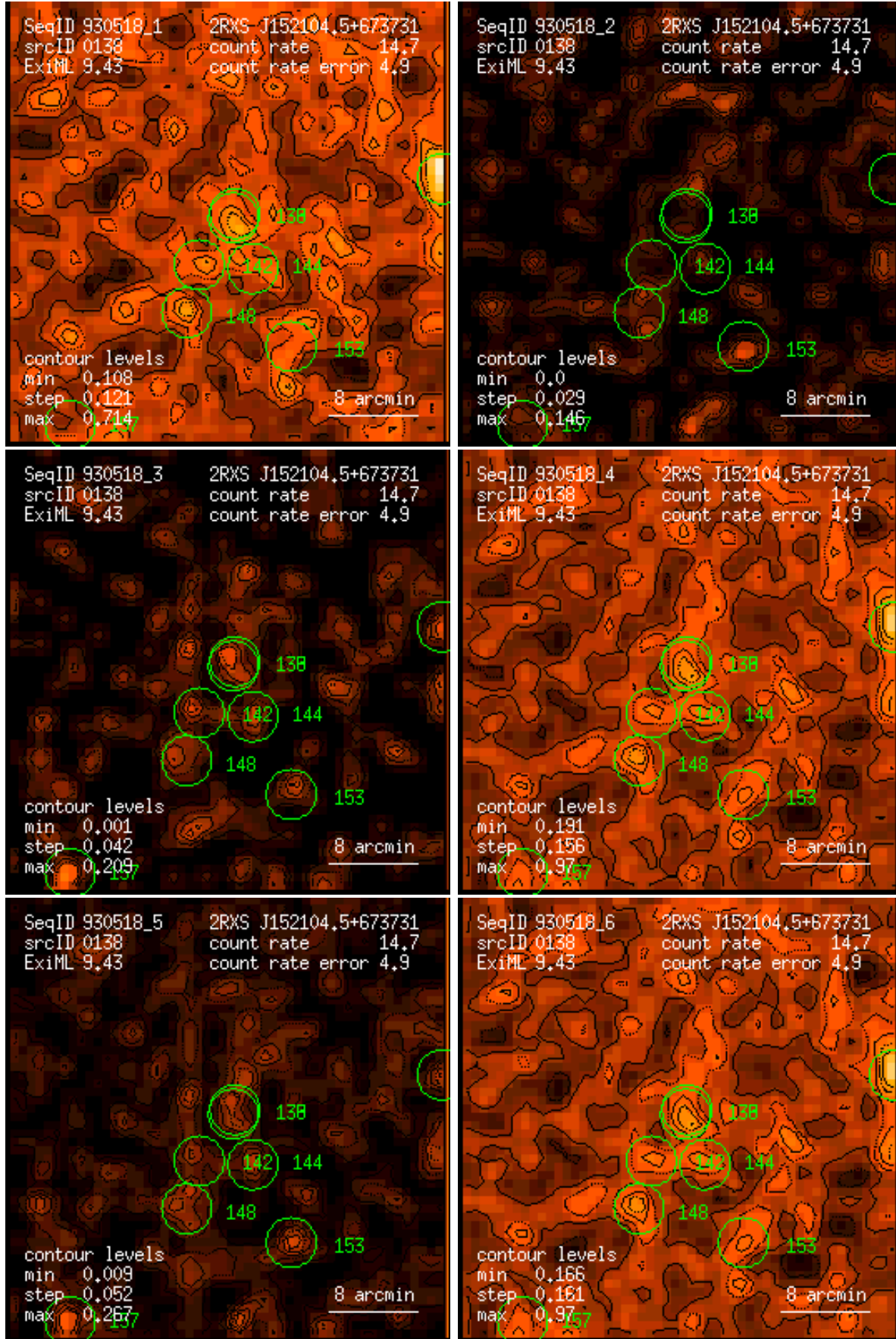
Figure 138: RASS 930518: detection 0138: band rate images, Gaussian filter: (1) PSPC channels 11 – 41, (2) 52 – 90, (3) 91 – 201, (4) 11 – 235, (5) 52 – 201, (6) 11 – 201. Broad band rates in counts/ks. Band rate contour levels in counts/ks/arcmin 2 .
