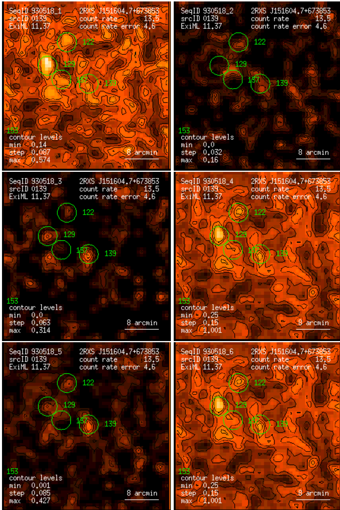
Figure 139: RASS 930518: detection 0139: band rate images, Gaussian filter: (1) PSPC channels 11 – 41, (2) 52 – 90, (3) 91 – 201, (4) 11 – 235, (5) 52 – 201, (6) 11 – 201. Broad band rates in counts/ks. Band rate contour levels in counts/ks/arcmin 2 .
