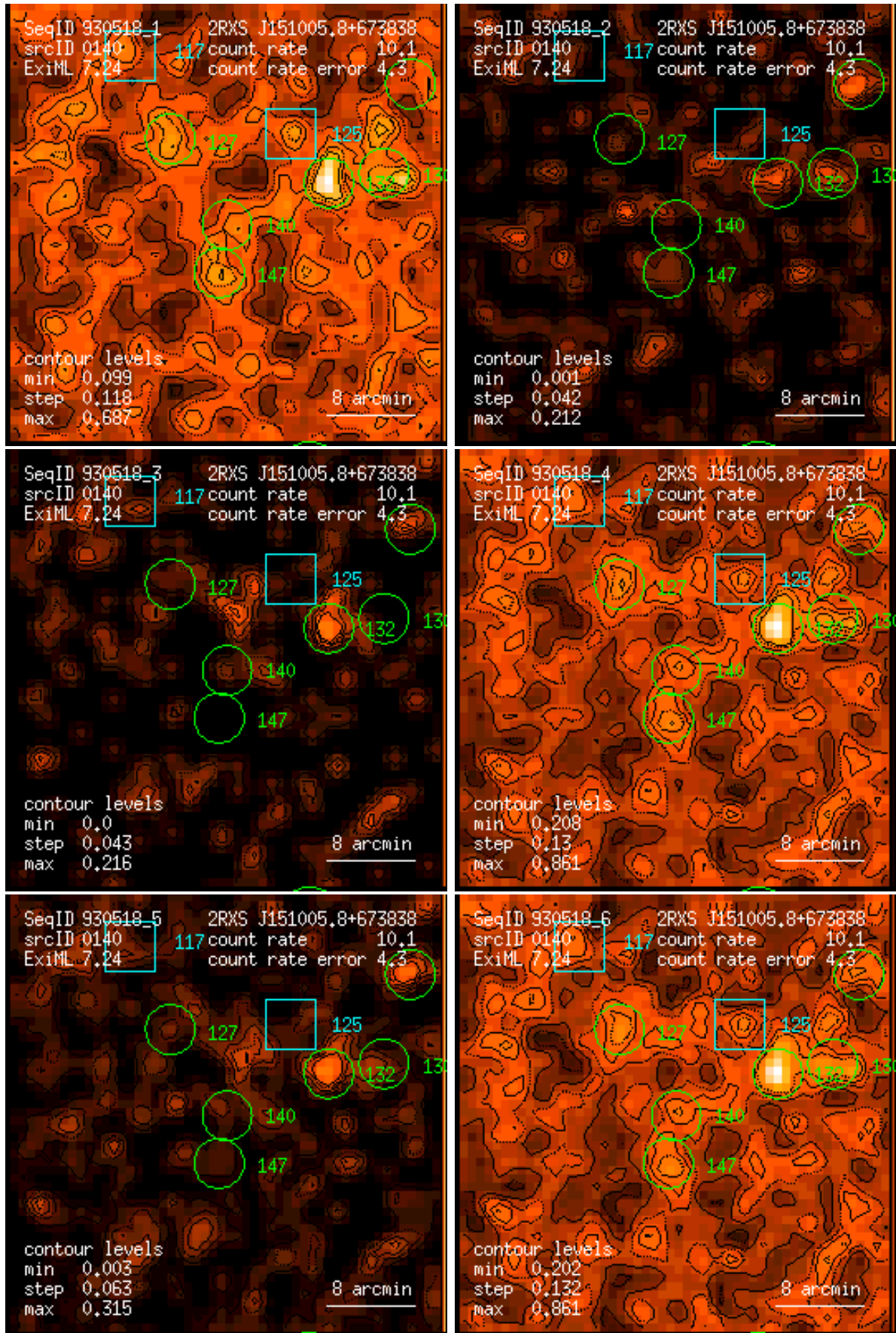
Figure 140: RASS 930518: detection 0140: band rate images, Gaussian filter: (1) PSPC channels 11 – 41, (2) 52 – 90, (3) 91 – 201, (4) 11 – 235, (5) 52 – 201, (6) 11 – 201. Broad band rates in counts/ks. Band rate contour levels in counts/ks/arcmin 2 .
