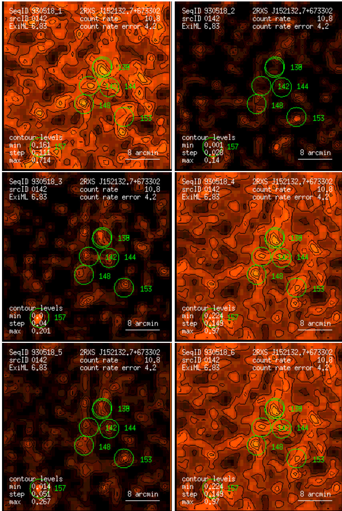
Figure 142: RASS 930518: detection 0142: band rate images, Gaussian filter: (1) PSPC channels 11 – 41, (2) 52 – 90, (3) 91 – 201, (4) 11 – 235, (5) 52 – 201, (6) 11 – 201. Broad band rates in counts/ks. Band rate contour levels in counts/ks/arcmin 2 .
