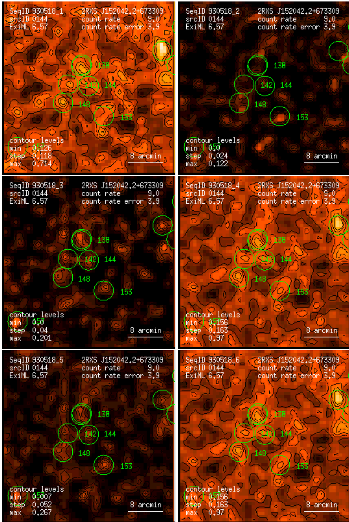
Figure 144: RASS 930518: detection 0144: band rate images, Gaussian filter: (1) PSPC channels 11 – 41, (2) 52 – 90, (3) 91 – 201, (4) 11 – 235, (5) 52 – 201, (6) 11 – 201. Broad band rates in counts/ks. Band rate contour levels in counts/ks/arcmin 2 .
