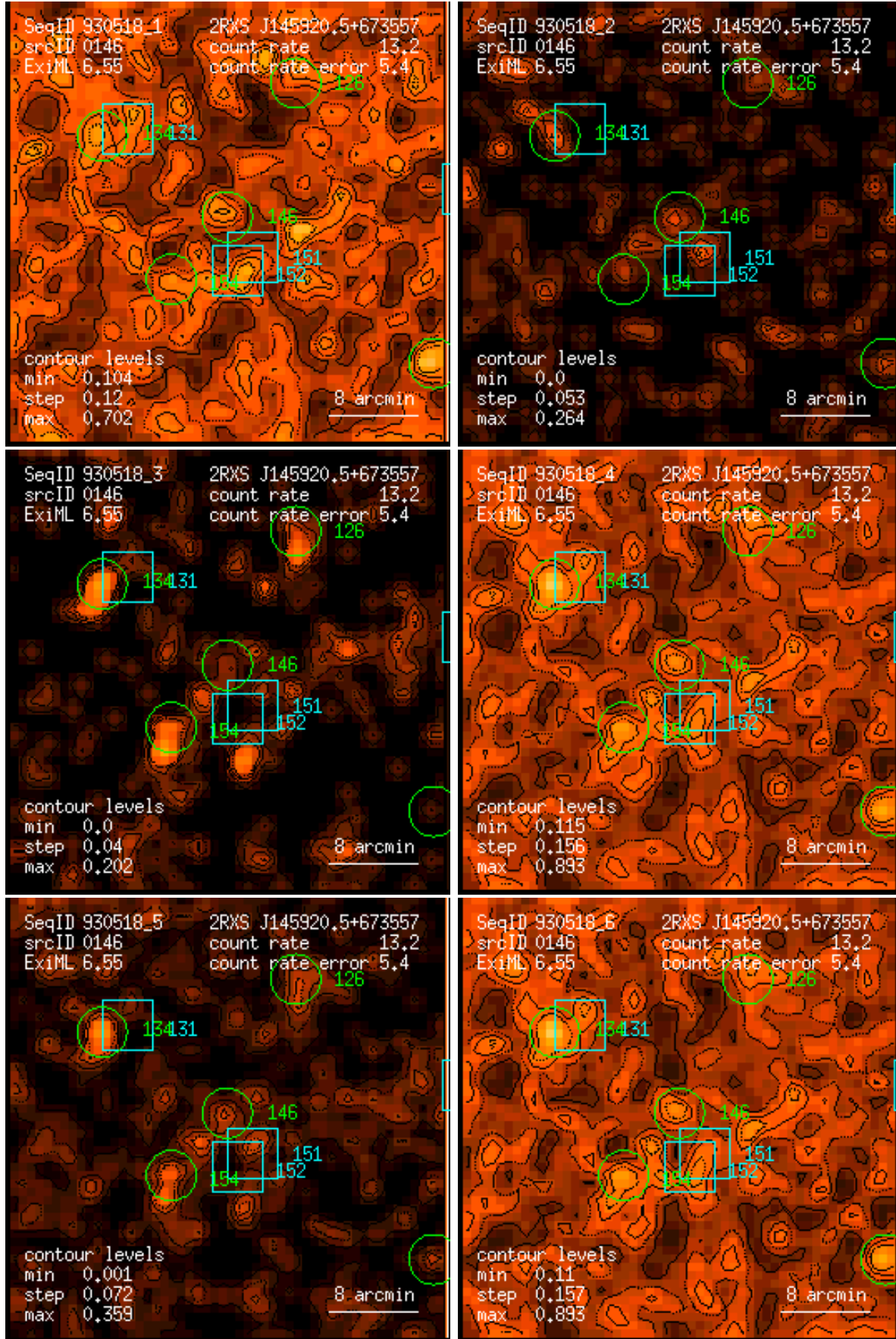
Figure 146: RASS 930518: detection 0146: band rate images, Gaussian filter: (1) PSPC channels 11 – 41, (2) 52 – 90, (3) 91 – 201, (4) 11 – 235, (5) 52 – 201, (6) 11 – 201. Broad band rates in counts/ks. Band rate contour levels in counts/ks/arcmin 2 .
