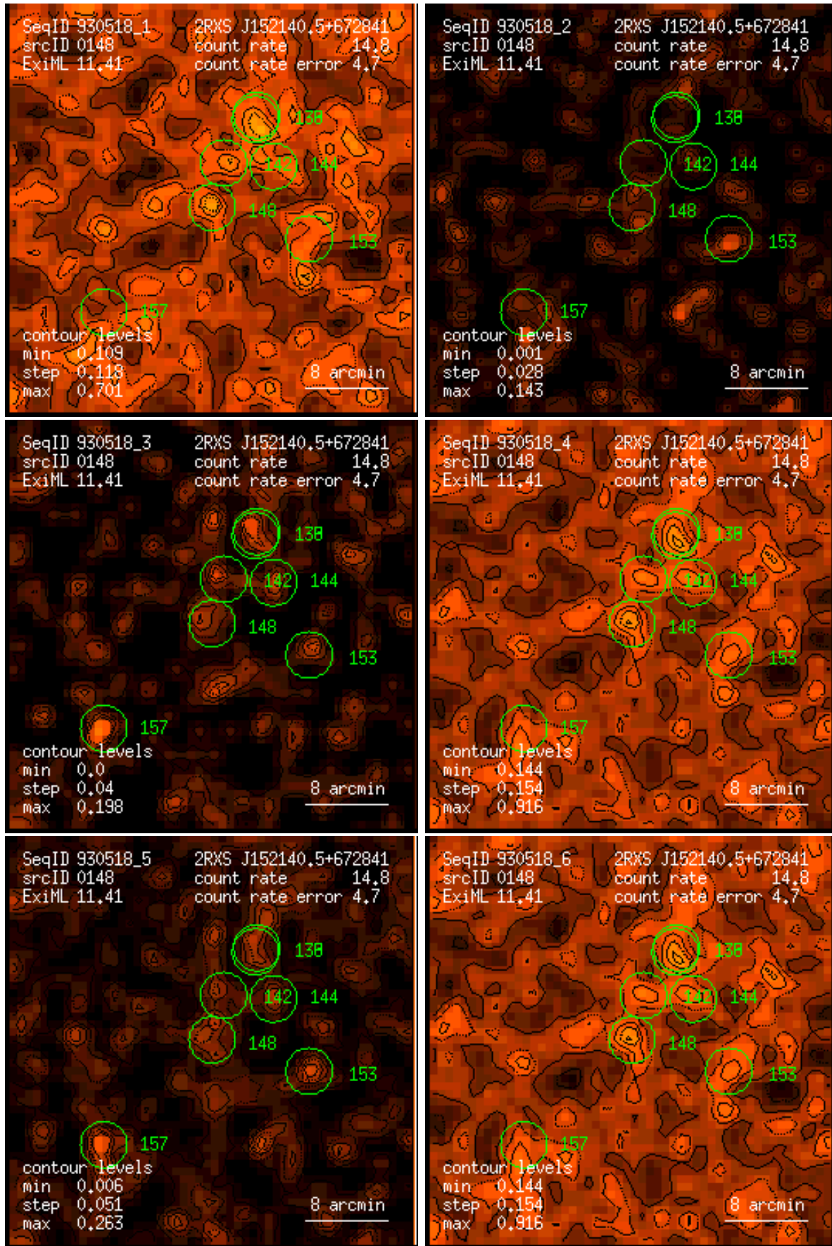
Figure 148: RASS 930518: detection 0148: band rate images, Gaussian filter: (1) PSPC channels 11 – 41, (2) 52 – 90, (3) 91 – 201, (4) 11 – 235, (5) 52 – 201, (6) 11 – 201. Broad band rates in counts/ks. Band rate contour levels in counts/ks/arcmin 2 .
