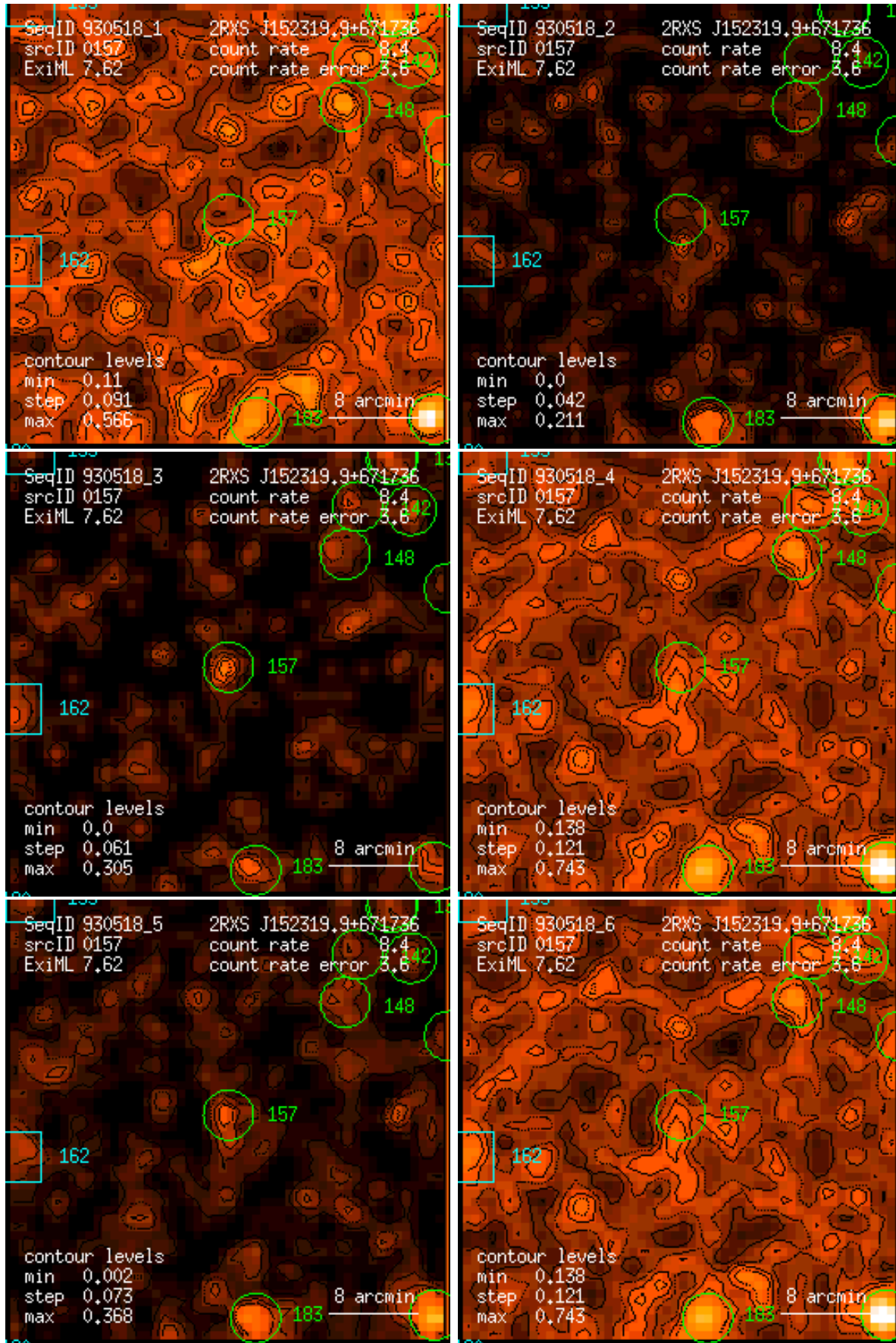
Figure 157: RASS 930518: detection 0157: band rate images, Gaussian filter: (1) PSPC channels 11 – 41, (2) 52 – 90, (3) 91 – 201, (4) 11 – 235, (5) 52 – 201, (6) 11 – 201. Broad band rates in counts/ks. Band rate contour levels in counts/ks/arcmin 2 .
