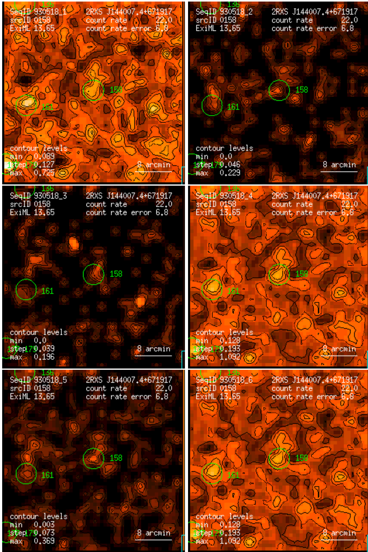
Figure 158: RASS 930518: detection 0158: band rate images, Gaussian filter: (1) PSPC channels 11 – 41, (2) 52 – 90, (3) 91 – 201, (4) 11 – 235, (5) 52 – 201, (6) 11 – 201. Broad band rates in counts/ks. Band rate contour levels in counts/ks/arcmin 2 .
