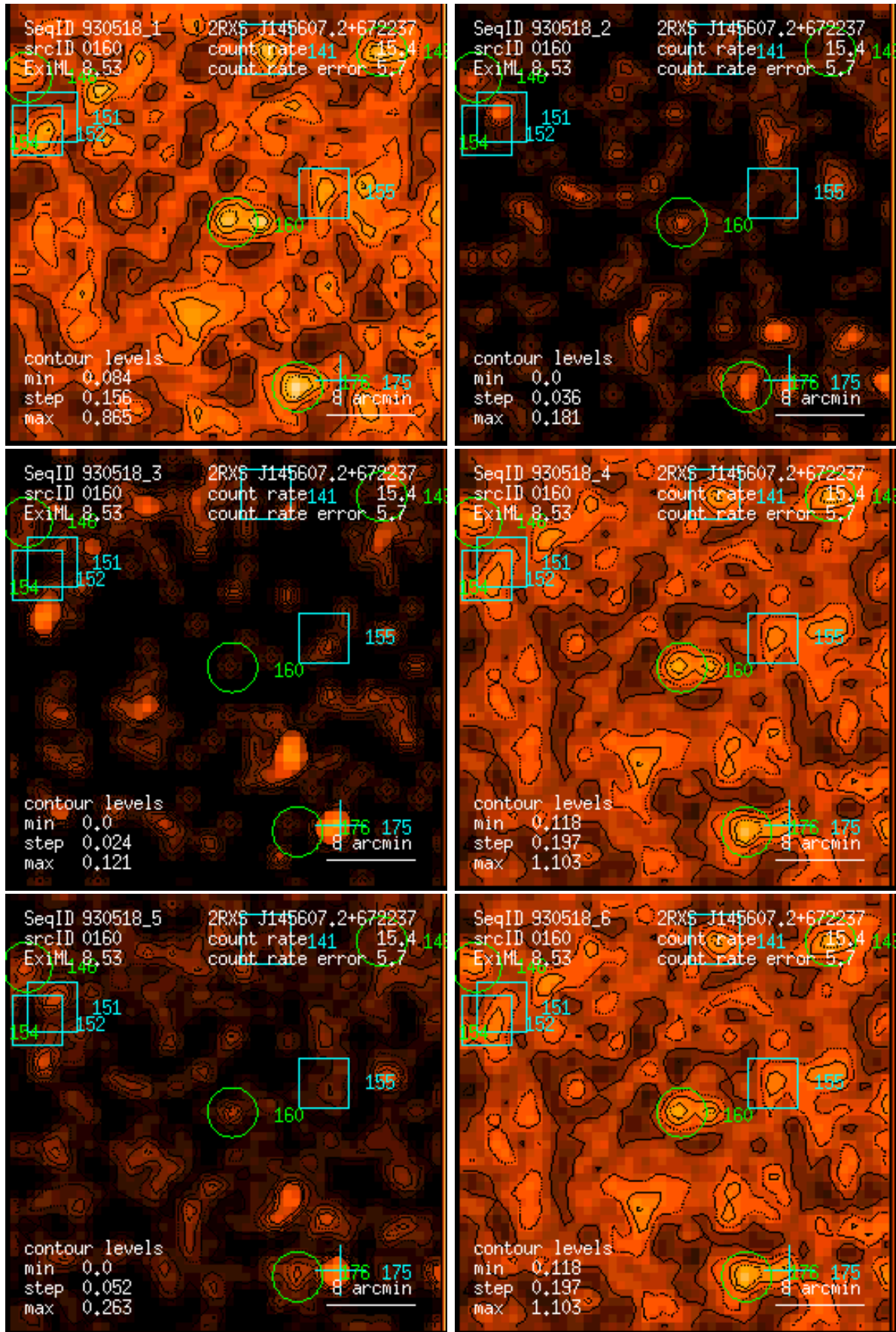
Figure 160: RASS 930518: detection 0160: band rate images, Gaussian filter: (1) PSPC channels 11 – 41, (2) 52 – 90, (3) 91 – 201, (4) 11 – 235, (5) 52 – 201, (6) 11 – 201. Broad band rates in counts/ks. Band rate contour levels in counts/ks/arcmin 2 .
