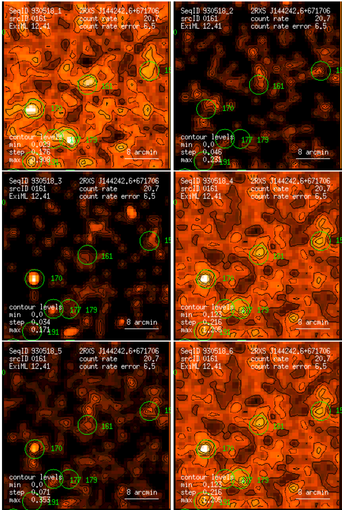
Figure 161: RASS 930518: detection 0161: band rate images, Gaussian filter: (1) PSPC channels 11 – 41, (2) 52 – 90, (3) 91 – 201, (4) 11 – 235, (5) 52 – 201, (6) 11 – 201. Broad band rates in counts/ks. Band rate contour levels in counts/ks/arcmin 2 .
