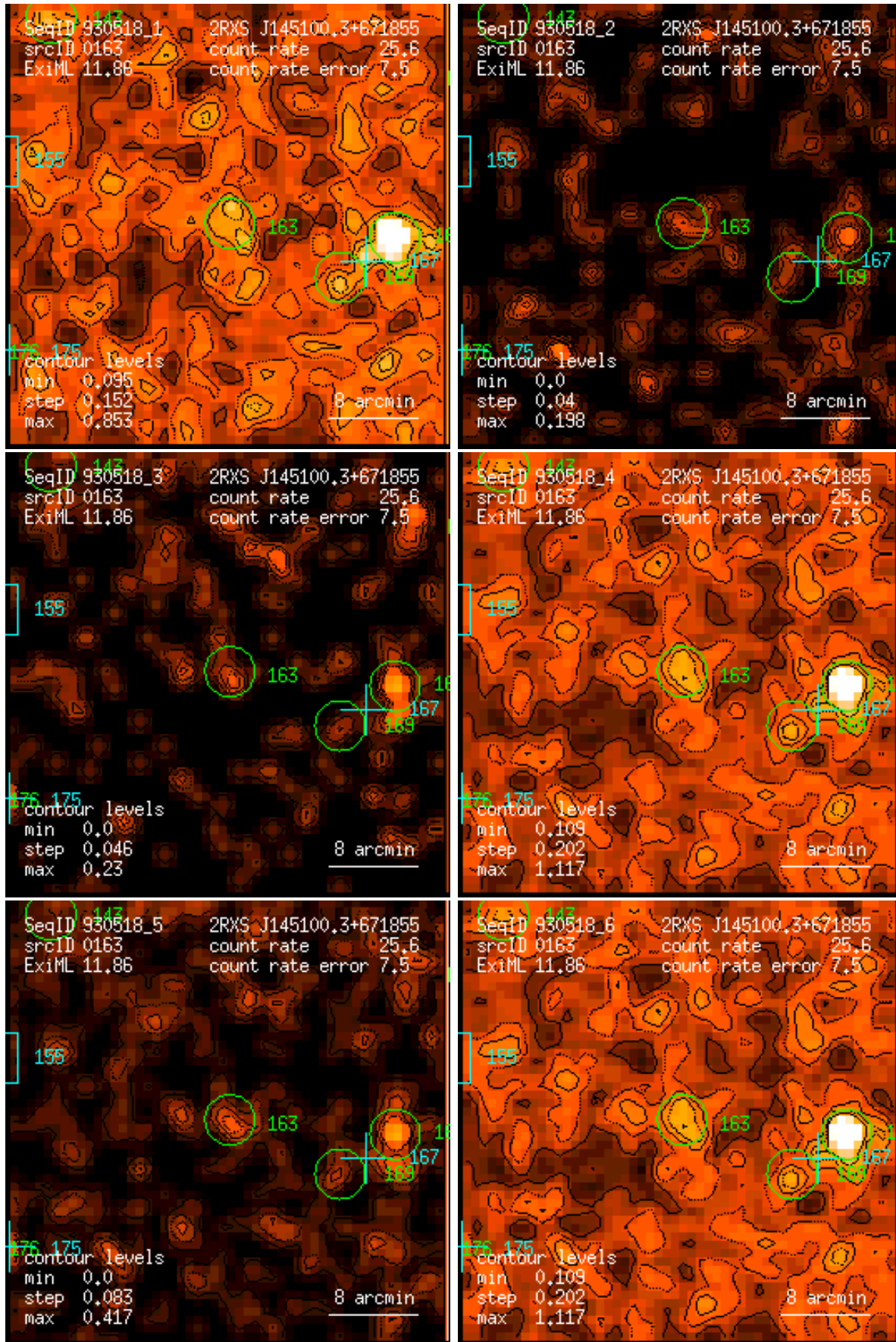
Figure 163: RASS 930518: detection 0163: band rate images, Gaussian filter: (1) PSPC channels 11 – 41, (2) 52 – 90, (3) 91 – 201, (4) 11 – 235, (5) 52 – 201, (6) 11 – 201. Broad band rates in counts/ks. Band rate contour levels in counts/ks/arcmin 2 .
