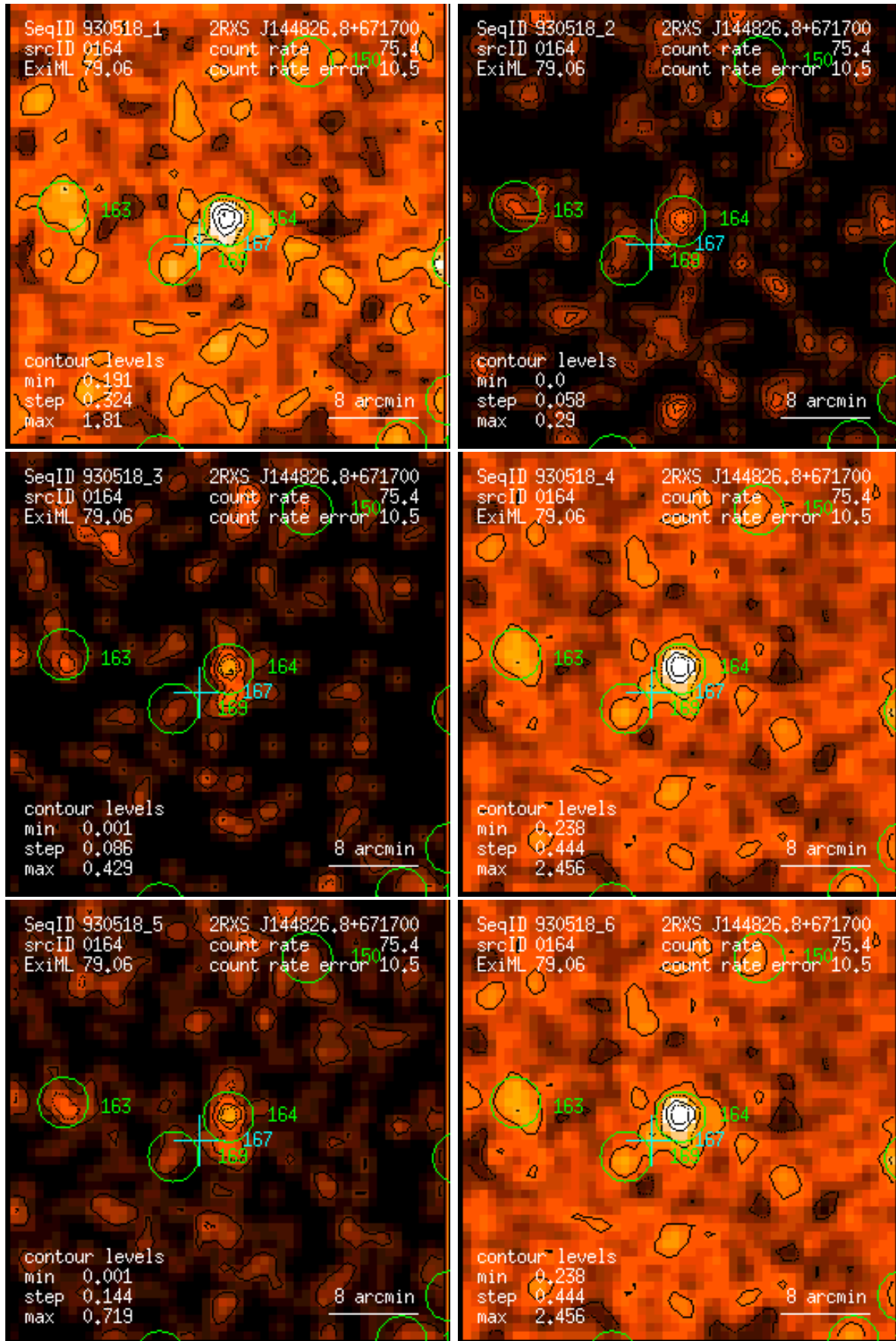
Figure 164: RASS 930518: detection 0164: band rate images, Gaussian filter: (1) PSPC channels 11 – 41, (2) 52 – 90, (3) 91 – 201, (4) 11 – 235, (5) 52 – 201, (6) 11 – 201. Broad band rates in counts/ks. Band rate contour levels in counts/ks/arcmin 2 .
