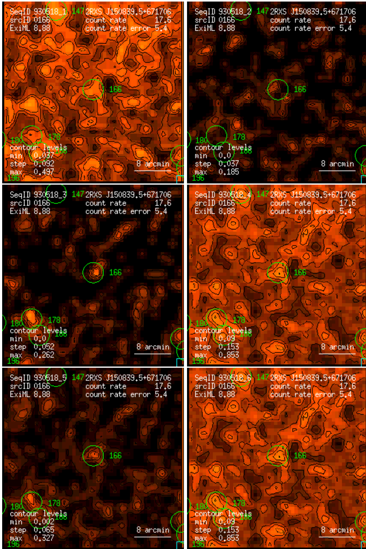
Figure 166: RASS 930518: detection 0166: band rate images, Gaussian filter: (1) PSPC channels 11 – 41, (2) 52 – 90, (3) 91 – 201, (4) 11 – 235, (5) 52 – 201, (6) 11 – 201. Broad band rates in counts/ks. Band rate contour levels in counts/ks/arcmin 2 .
