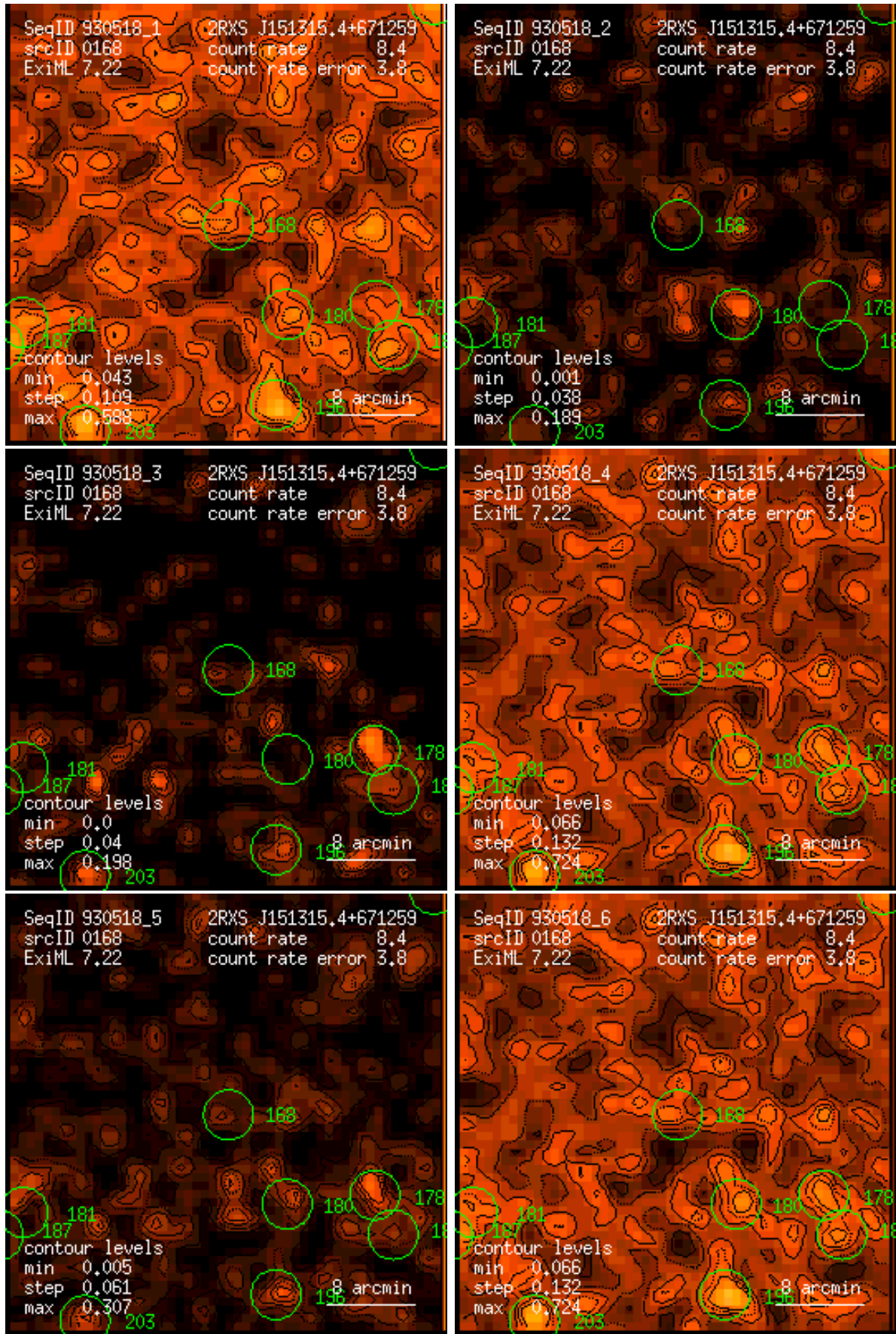
Figure 168: RASS 930518: detection 0168: band rate images, Gaussian filter: (1) PSPC channels 11 – 41, (2) 52 – 90, (3) 91 – 201, (4) 11 – 235, (5) 52 – 201, (6) 11 – 201. Broad band rates in counts/ks. Band rate contour levels in counts/ks/arcmin 2 .
