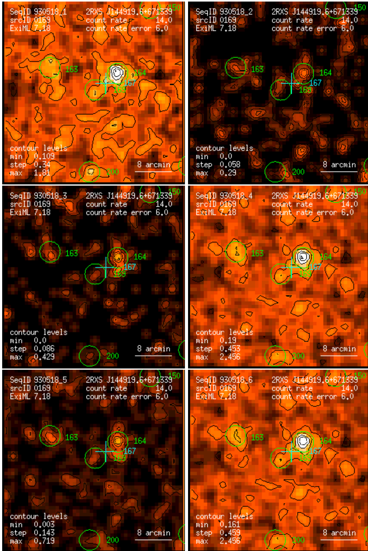
Figure 169: RASS 930518: detection 0169: band rate images, Gaussian filter: (1) PSPC channels 11 – 41, (2) 52 – 90, (3) 91 – 201, (4) 11 – 235, (5) 52 – 201, (6) 11 – 201. Broad band rates in counts/ks. Band rate contour levels in counts/ks/arcmin 2 .
