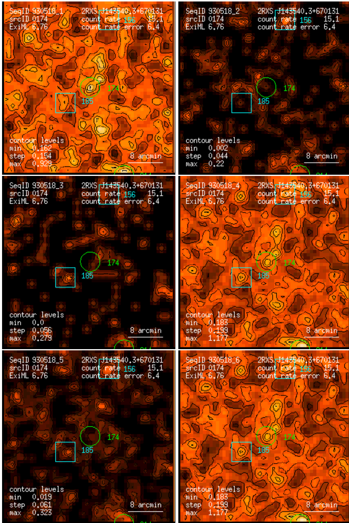
Figure 174: RASS 930518: detection 0174: band rate images, Gaussian filter: (1) PSPC channels 11 – 41, (2) 52 – 90, (3) 91 – 201, (4) 11 – 235, (5) 52 – 201, (6) 11 – 201. Broad band rates in counts/ks. Band rate contour levels in counts/ks/arcmin 2 .
