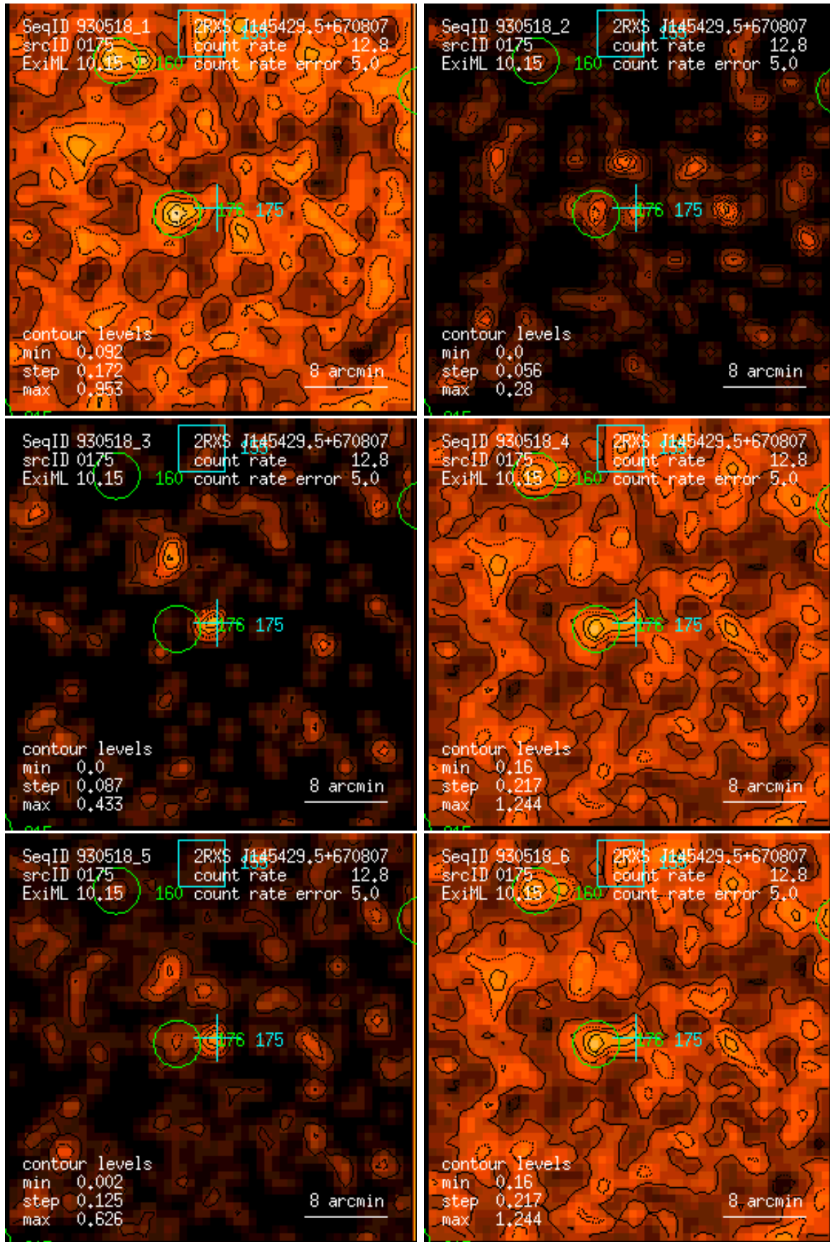
Figure 175: RASS 930518: detection 0175: band rate images, Gaussian filter: (1) PSPC channels 11 – 41, (2) 52 – 90, (3) 91 – 201, (4) 11 – 235, (5) 52 – 201, (6) 11 – 201. Broad band rates in counts/ks. Band rate contour levels in counts/ks/arcmin 2 .
