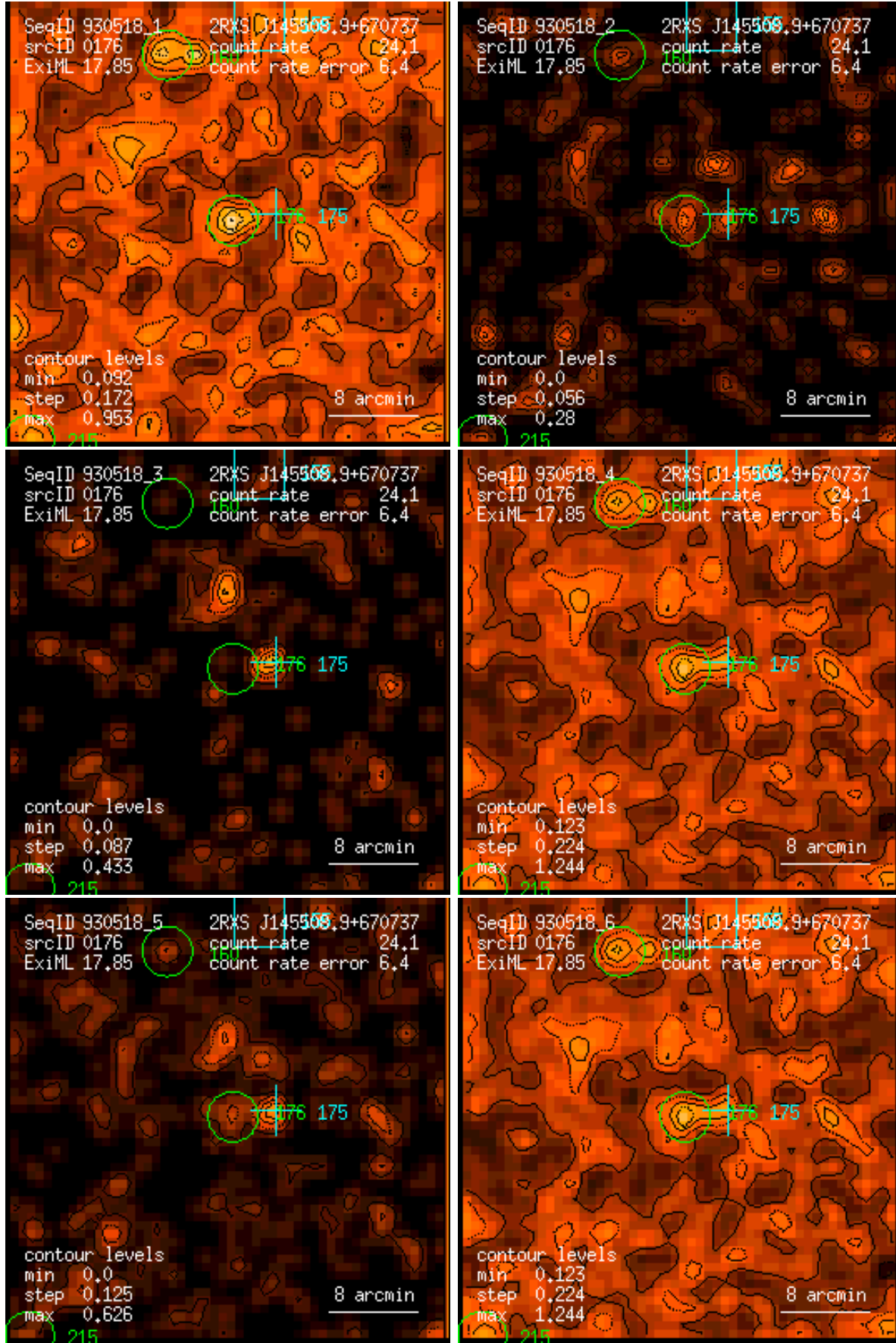
Figure 176: RASS 930518: detection 0176: band rate images, Gaussian filter: (1) PSPC channels 11 – 41, (2) 52 – 90, (3) 91 – 201, (4) 11 – 235, (5) 52 – 201, (6) 11 – 201. Broad band rates in counts/ks. Band rate contour levels in counts/ks/arcmin 2 .
