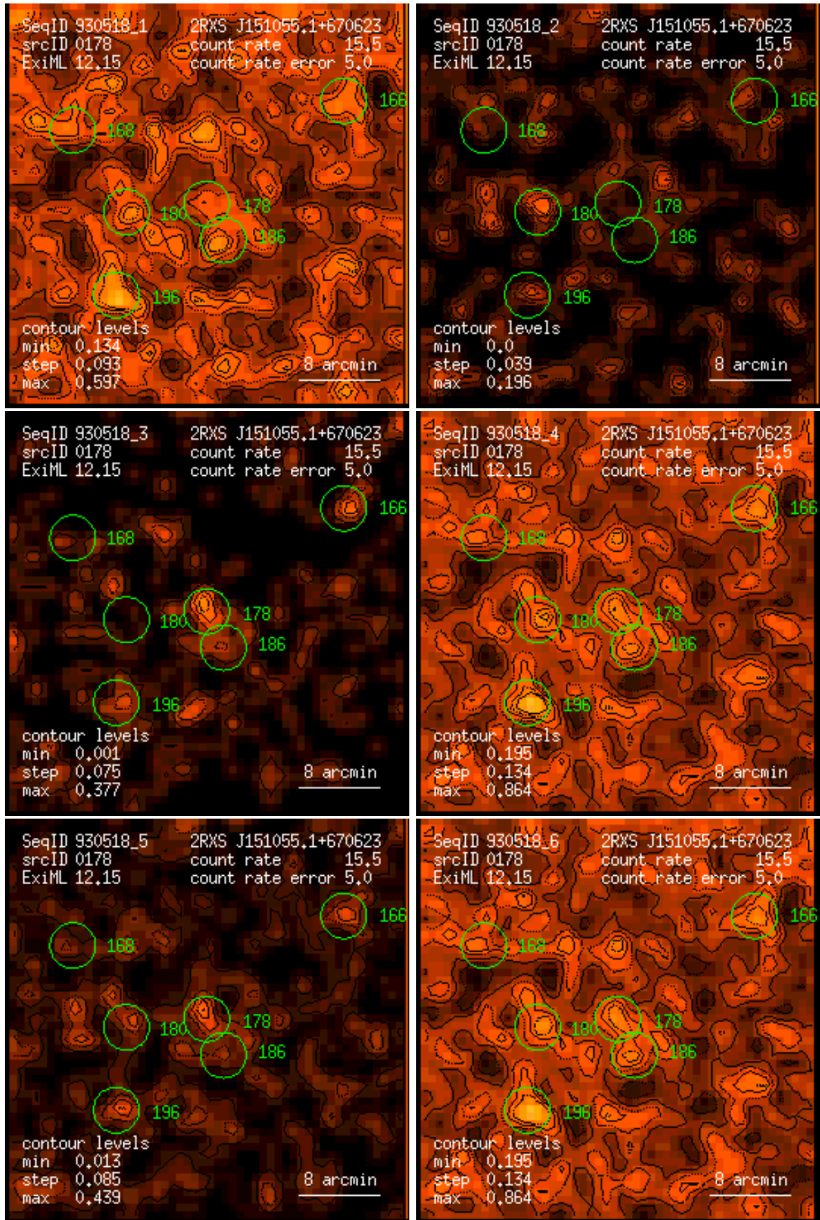
Figure 178: RASS 930518: detection 0178: band rate images, Gaussian filter: (1) PSPC channels 11 – 41, (2) 52 – 90, (3) 91 – 201, (4) 11 – 235, (5) 52 – 201, (6) 11 – 201. Broad band rates in counts/ks. Band rate contour levels in counts/ks/arcmin 2 .
