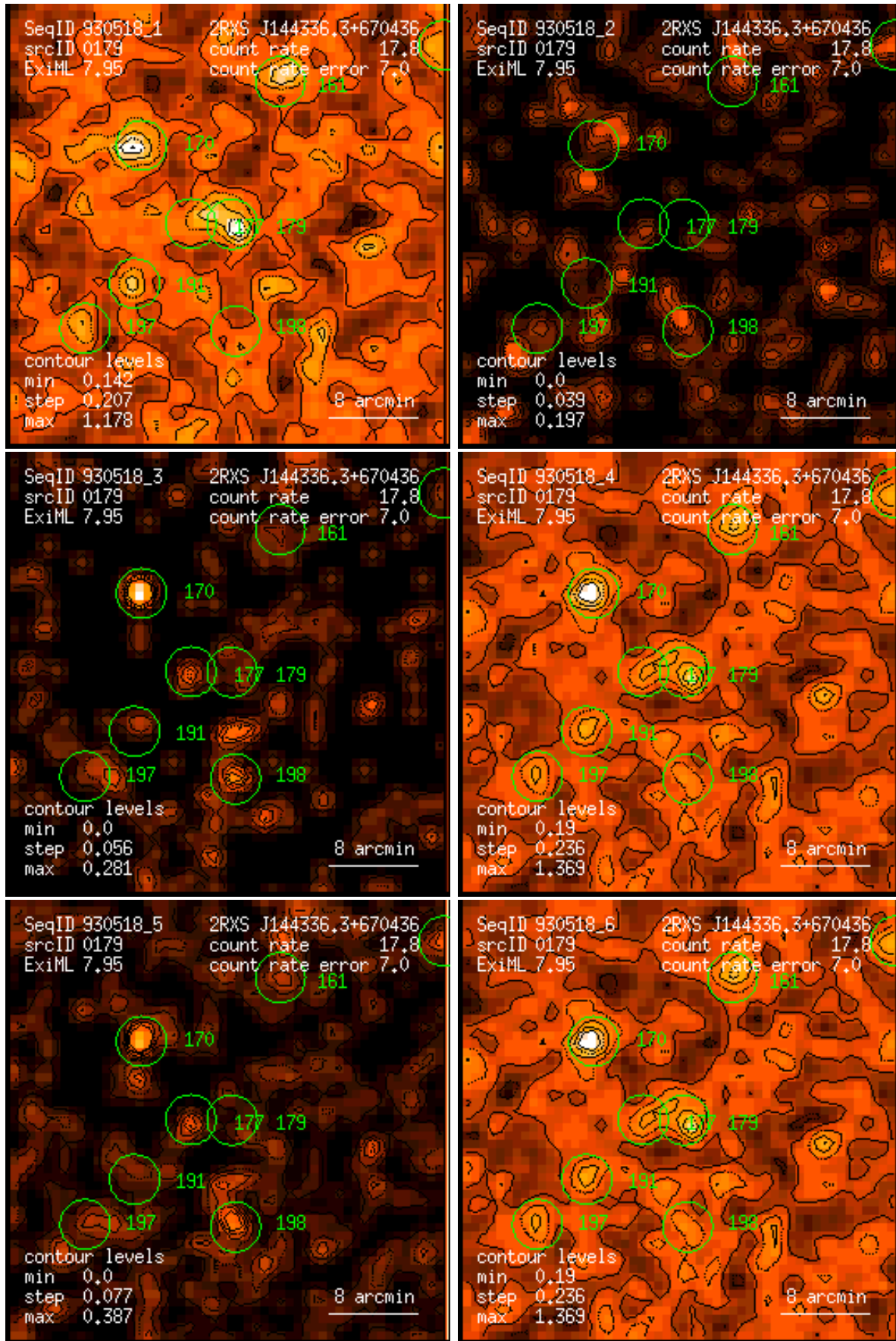
Figure 179: RASS 930518: detection 0179: band rate images, Gaussian filter: (1) PSPC channels 11 – 41, (2) 52 – 90, (3) 91 – 201, (4) 11 – 235, (5) 52 – 201, (6) 11 – 201. Broad band rates in counts/ks. Band rate contour levels in counts/ks/arcmin 2 .
