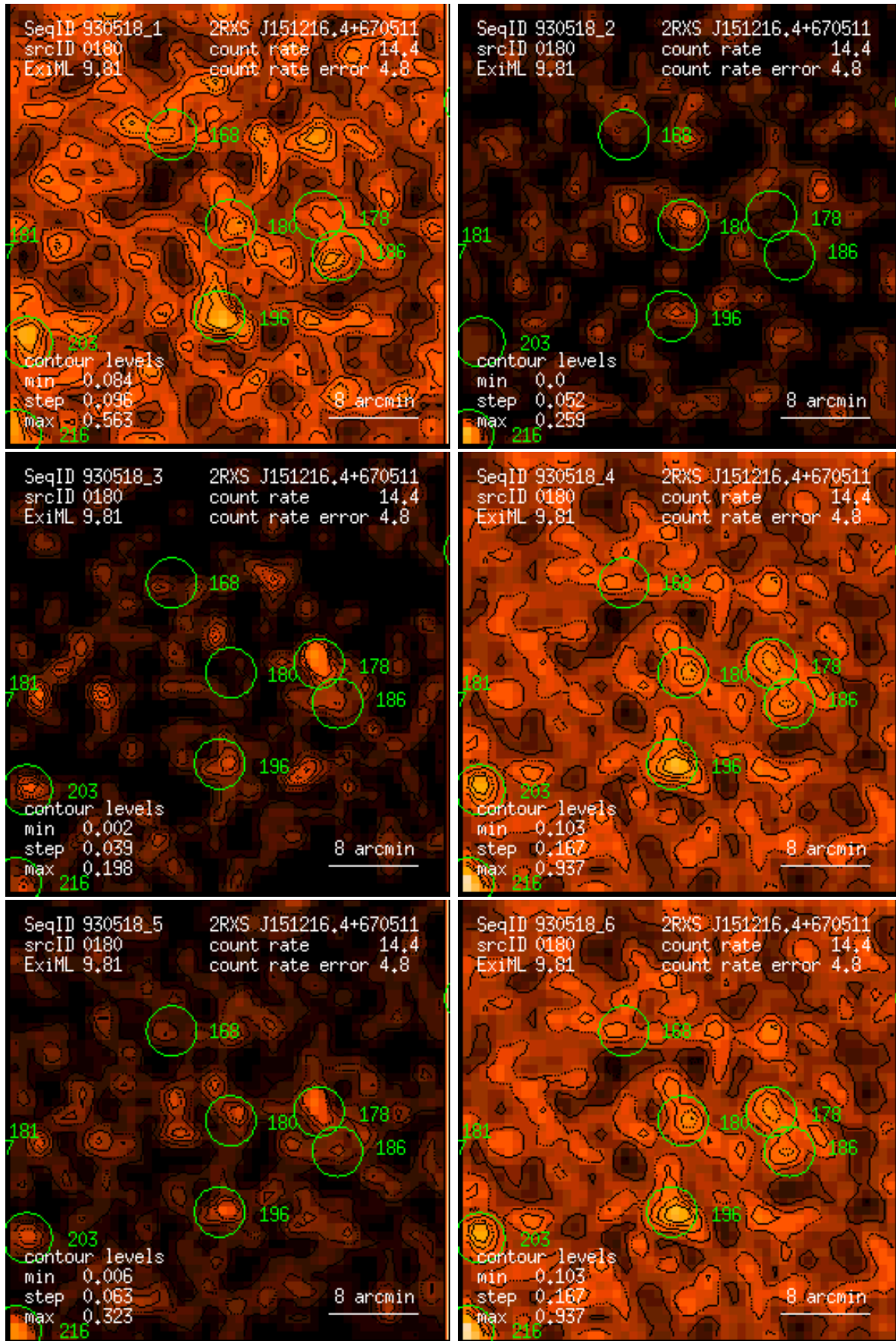
Figure 180: RASS 930518: detection 0180: band rate images, Gaussian filter: (1) PSPC channels 11 – 41, (2) 52 – 90, (3) 91 – 201, (4) 11 – 235, (5) 52 – 201, (6) 11 – 201. Broad band rates in counts/ks. Band rate contour levels in counts/ks/arcmin 2 .
