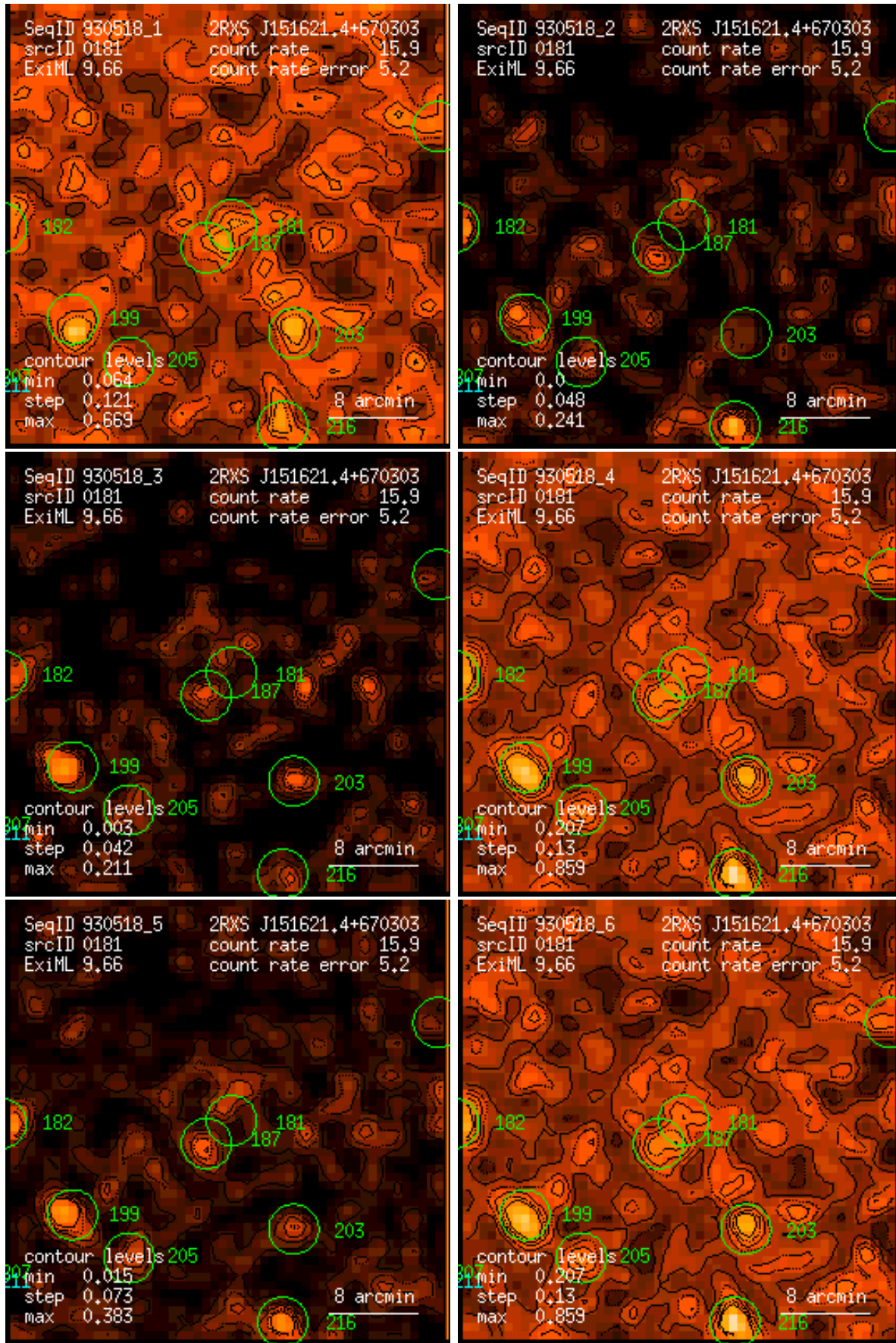
Figure 181: RASS 930518: detection 0181: band rate images, Gaussian filter: (1) PSPC channels 11 – 41, (2) 52 – 90, (3) 91 – 201, (4) 11 – 235, (5) 52 – 201, (6) 11 – 201. Broad band rates in counts/ks. Band rate contour levels in counts/ks/arcmin 2 .
