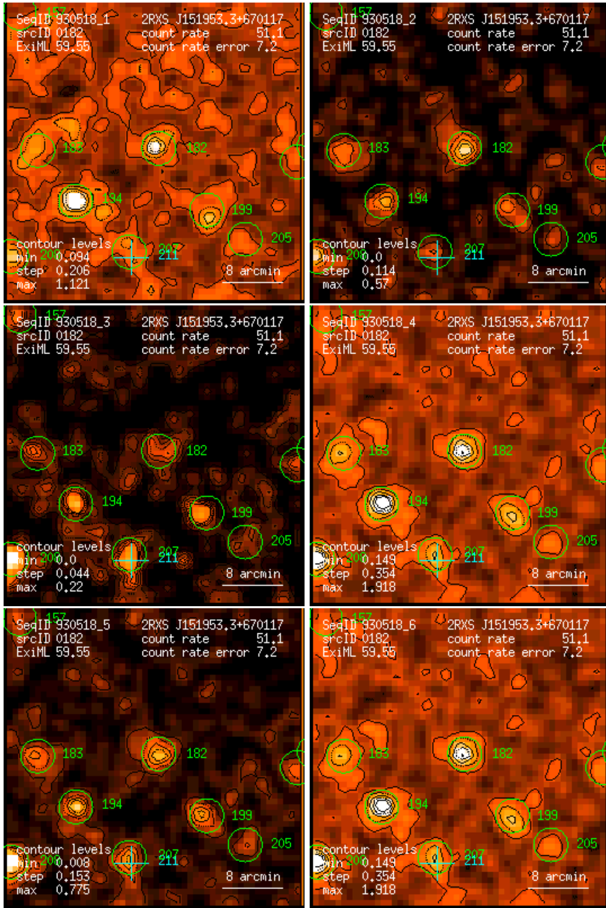
Figure 182: RASS 930518: detection 0182: band rate images, Gaussian filter: (1) PSPC channels 11 – 41, (2) 52 – 90, (3) 91 – 201, (4) 11 – 235, (5) 52 – 201, (6) 11 – 201. Broad band rates in counts/ks. Band rate contour levels in counts/ks/arcmin 2 .
