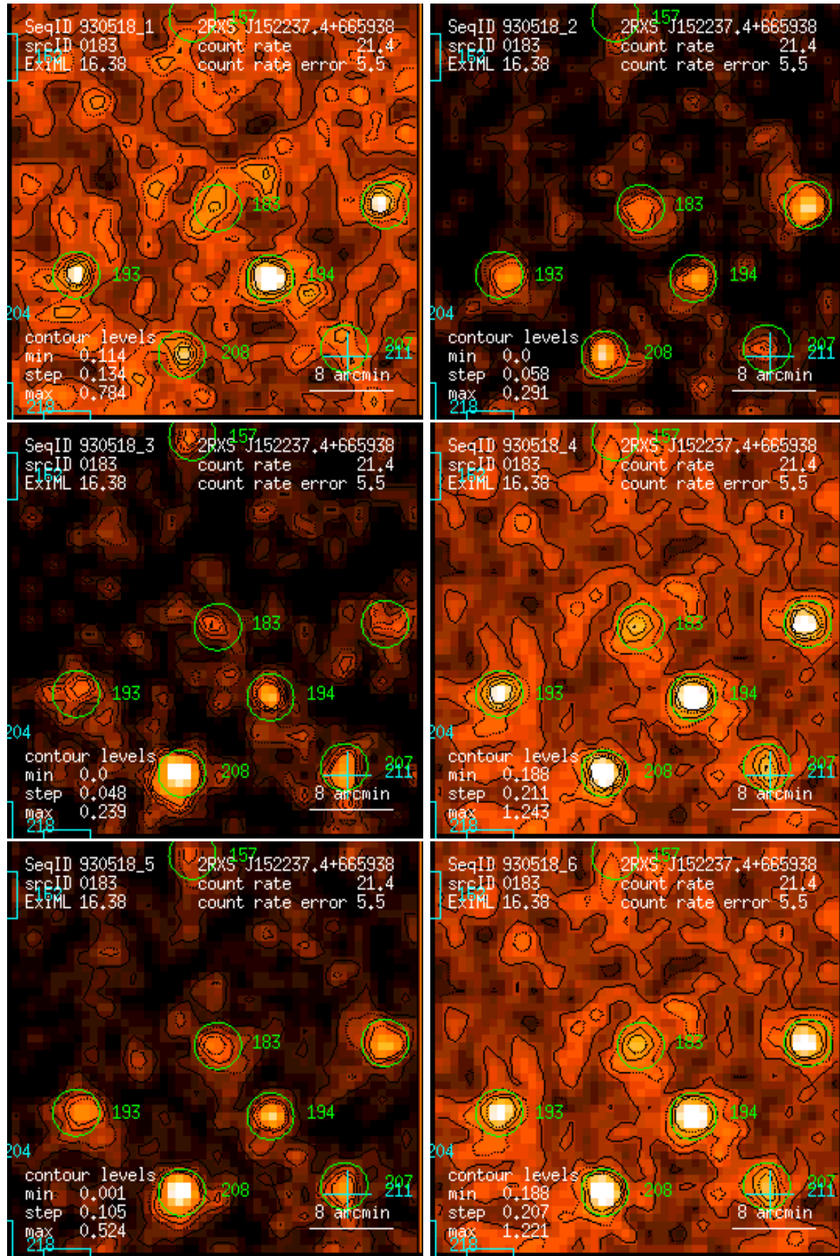
Figure 183: RASS 930518: detection 0183: band rate images, Gaussian filter: (1) PSPC channels 11 – 41, (2) 52 – 90, (3) 91 – 201, (4) 11 – 235, (5) 52 – 201, (6) 11 – 201. Broad band rates in counts/ks. Band rate contour levels in counts/ks/arcmin 2 .
