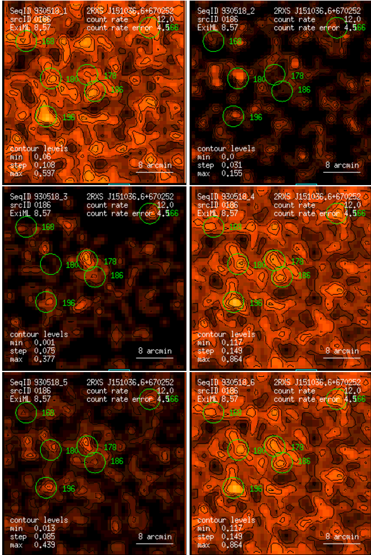
Figure 186: RASS 930518: detection 0186: band rate images, Gaussian filter: (1) PSPC channels 11 – 41, (2) 52 – 90, (3) 91 – 201, (4) 11 – 235, (5) 52 – 201, (6) 11 – 201. Broad band rates in counts/ks. Band rate contour levels in counts/ks/arcmin 2 .
