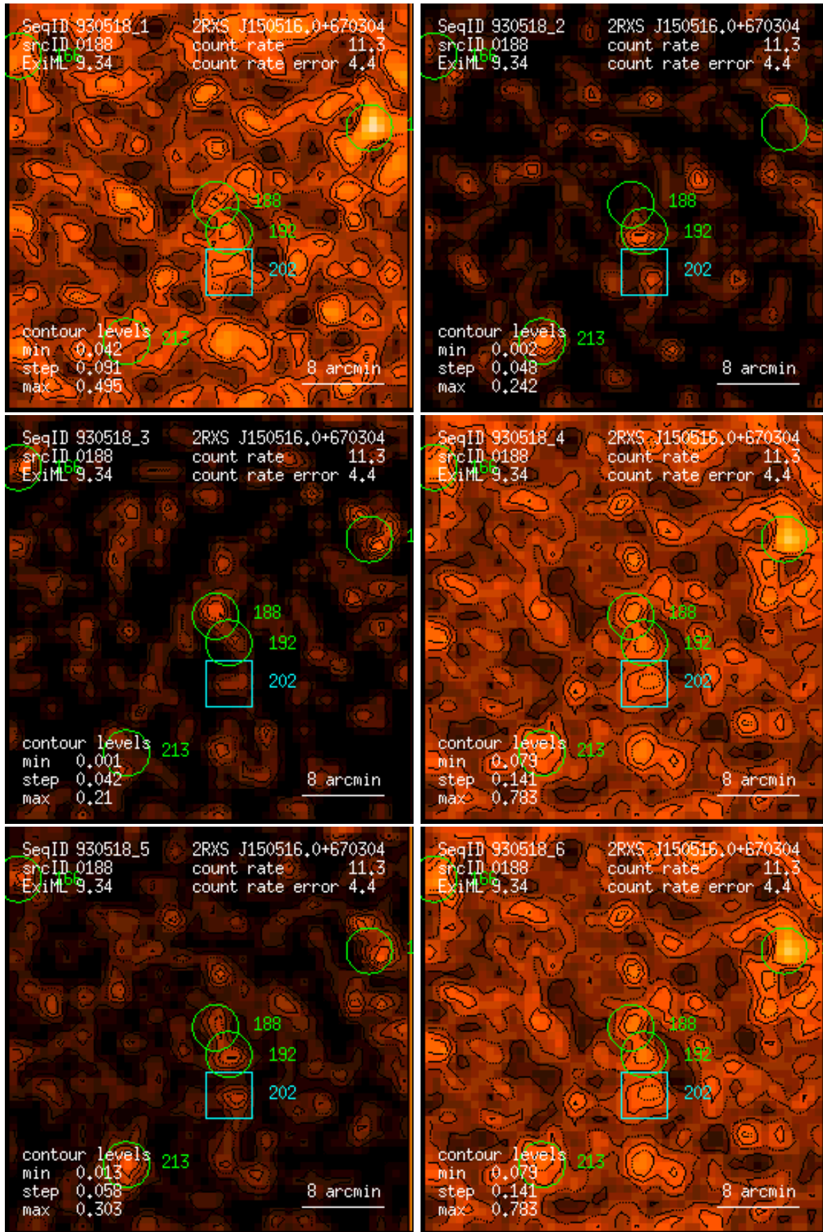
Figure 188: RASS 930518: detection 0188: band rate images, Gaussian filter: (1) PSPC channels 11 – 41, (2) 52 – 90, (3) 91 – 201, (4) 11 – 235, (5) 52 – 201, (6) 11 – 201. Broad band rates in counts/ks. Band rate contour levels in counts/ks/arcmin 2 .
