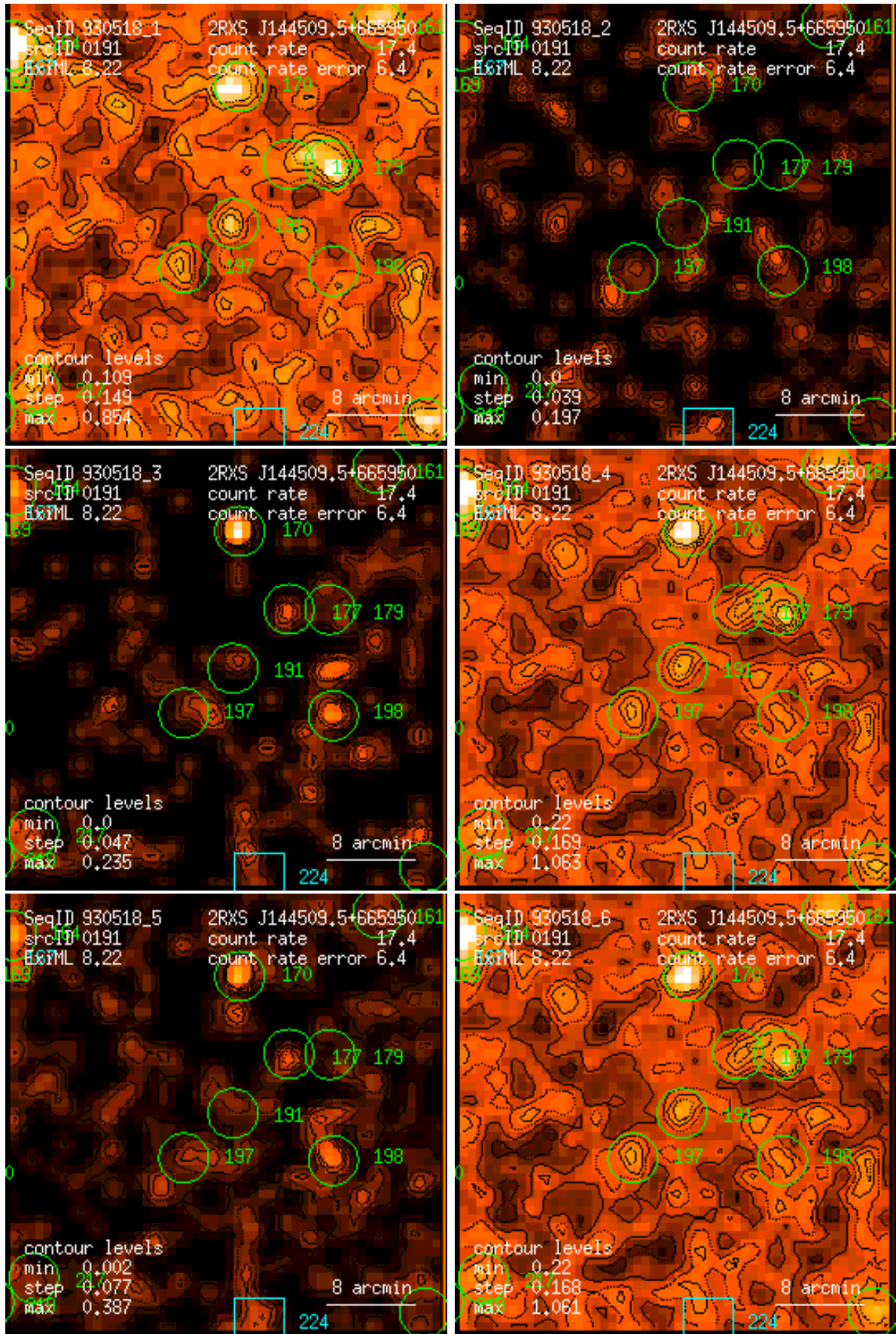
Figure 191: RASS 930518: detection 0191: band rate images, Gaussian filter: (1) PSPC channels 11 – 41, (2) 52 – 90, (3) 91 – 201, (4) 11 – 235, (5) 52 – 201, (6) 11 – 201. Broad band rates in counts/ks. Band rate contour levels in counts/ks/arcmin 2 .
