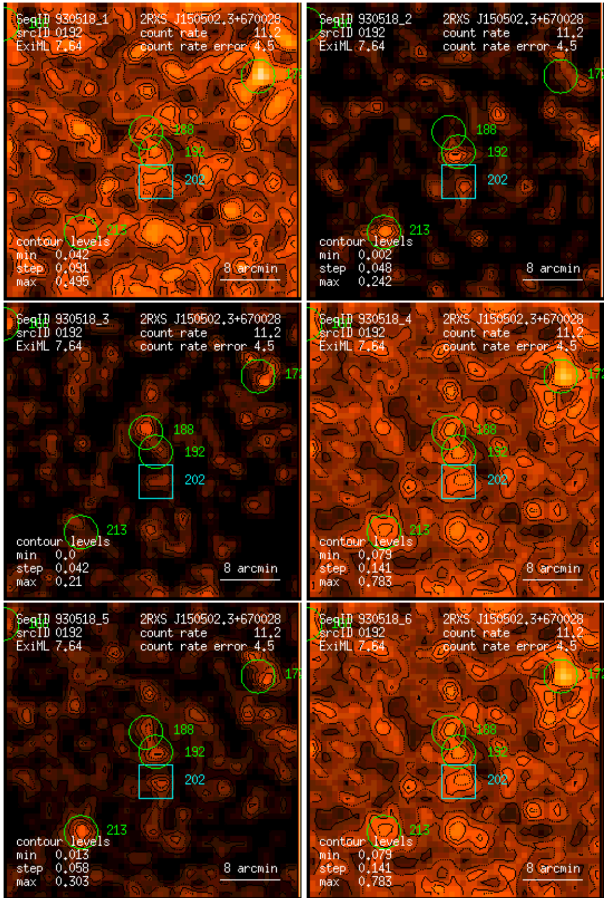
Figure 192: RASS 930518: detection 0192: band rate images, Gaussian filter: (1) PSPC channels 11 – 41, (2) 52 – 90, (3) 91 – 201, (4) 11 – 235, (5) 52 – 201, (6) 11 – 201. Broad band rates in counts/ks. Band rate contour levels in counts/ks/arcmin 2 .
