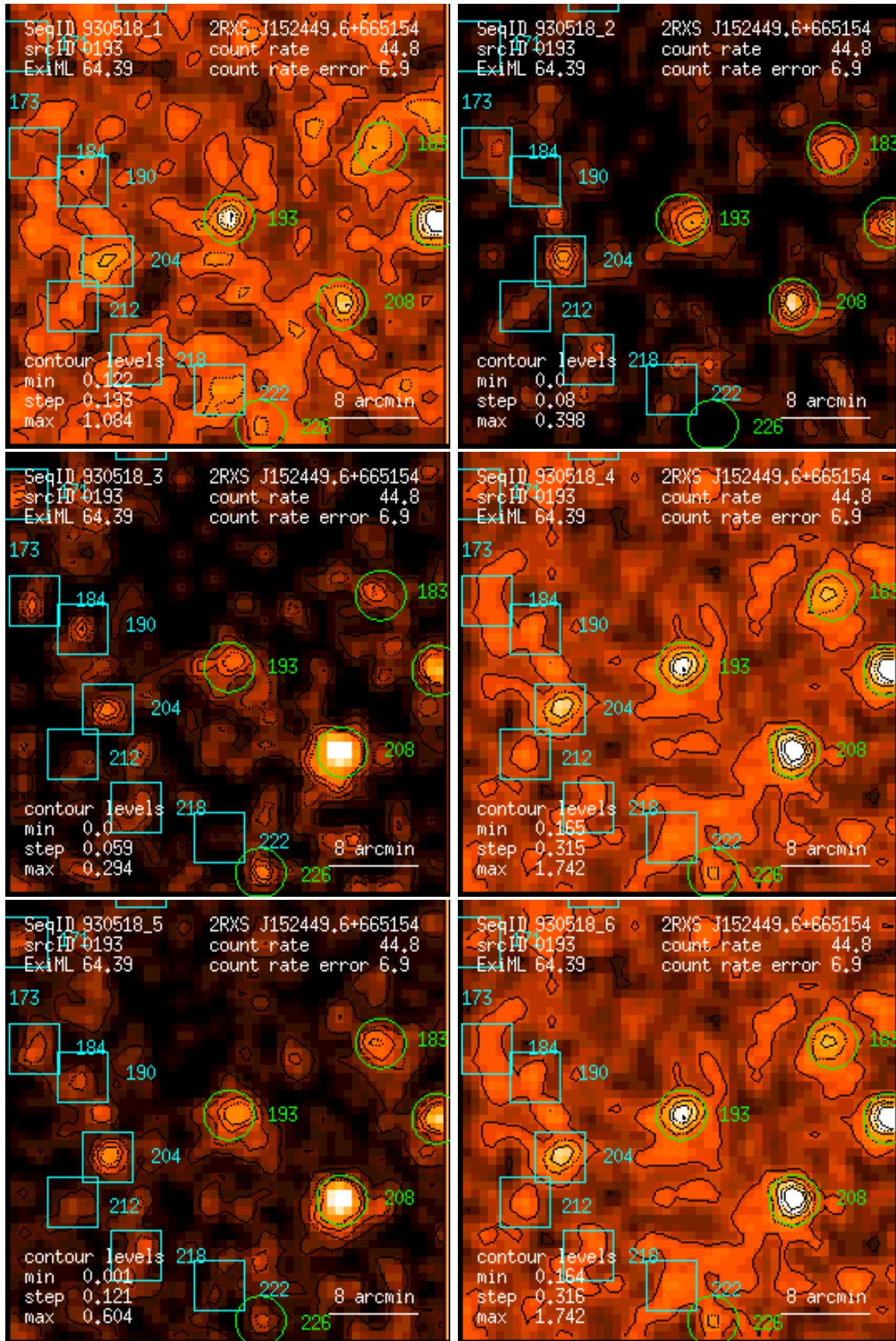
Figure 193: RASS 930518: detection 0193: band rate images, Gaussian filter: (1) PSPC channels 11 – 41, (2) 52 – 90, (3) 91 – 201, (4) 11 – 235, (5) 52 – 201, (6) 11 – 201. Broad band rates in counts/ks. Band rate contour levels in counts/ks/arcmin 2 .
