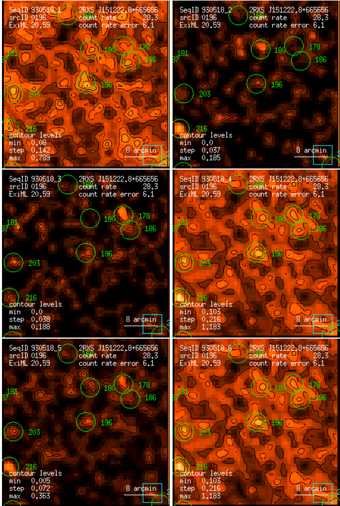
Figure 196: RASS 930518: detection 0196: band rate images, Gaussian filter: (1) PSPC channels 11 – 41, (2) 52 – 90, (3) 91 – 201, (4) 11 – 235, (5) 52 – 201, (6) 11 – 201. Broad band rates in counts/ks. Band rate contour levels in counts/ks/arcmin 2 .
