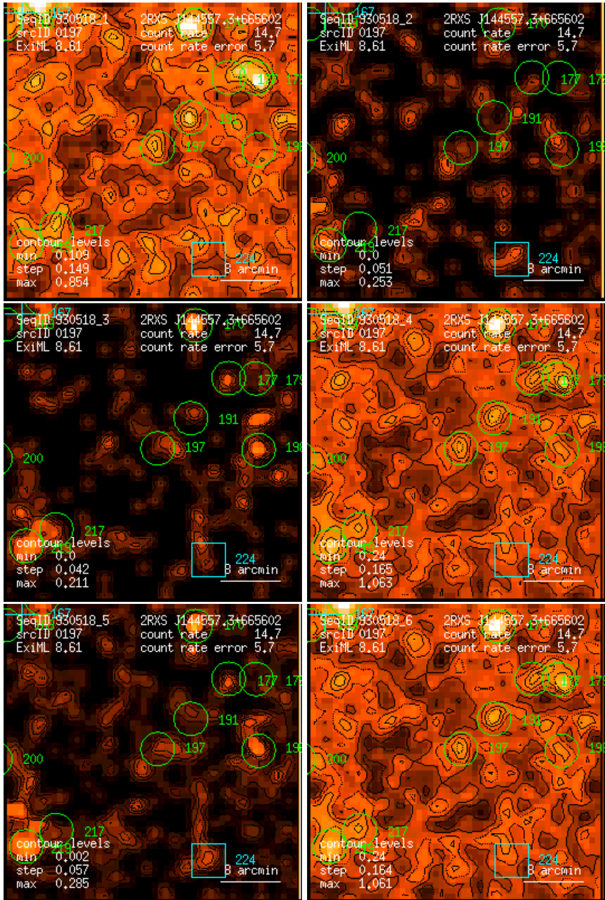
Figure 197: RASS 930518: detection 0197: band rate images, Gaussian filter: (1) PSPC channels 11 – 41, (2) 52 – 90, (3) 91 – 201, (4) 11 – 235, (5) 52 – 201, (6) 11 – 201. Broad band rates in counts/ks. Band rate contour levels in counts/ks/arcmin 2 .
