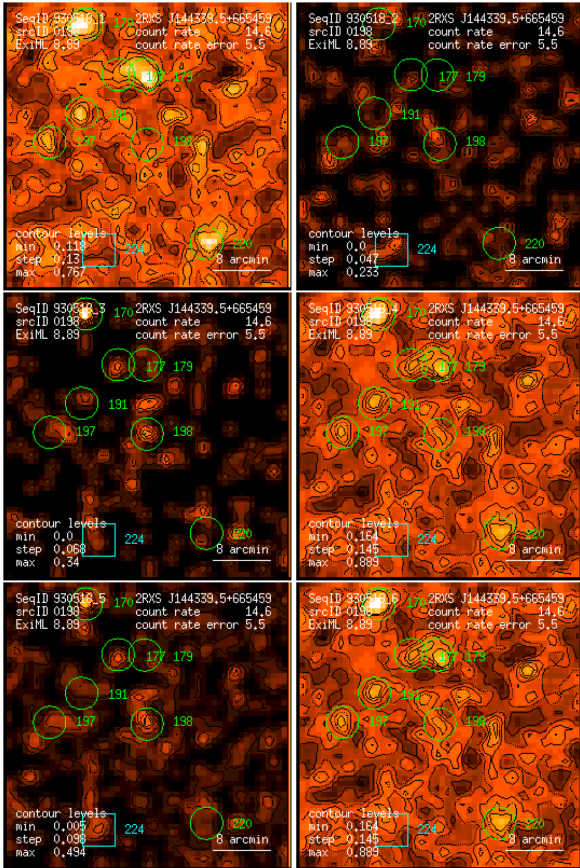
Figure 198: RASS 930518: detection 0198: band rate images, Gaussian filter: (1) PSPC channels 11 – 41, (2) 52 – 90, (3) 91 – 201, (4) 11 – 235, (5) 52 – 201, (6) 11 – 201. Broad band rates in counts/ks. Band rate contour levels in counts/ks/arcmin 2 .
