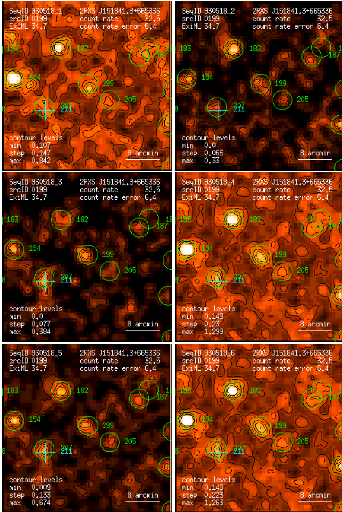
Figure 199: RASS 930518: detection 0199: band rate images, Gaussian filter: (1) PSPC channels 11 – 41, (2) 52 – 90, (3) 91 – 201, (4) 11 – 235, (5) 52 – 201, (6) 11 – 201. Broad band rates in counts/ks. Band rate contour levels in counts/ks/arcmin 2 .
