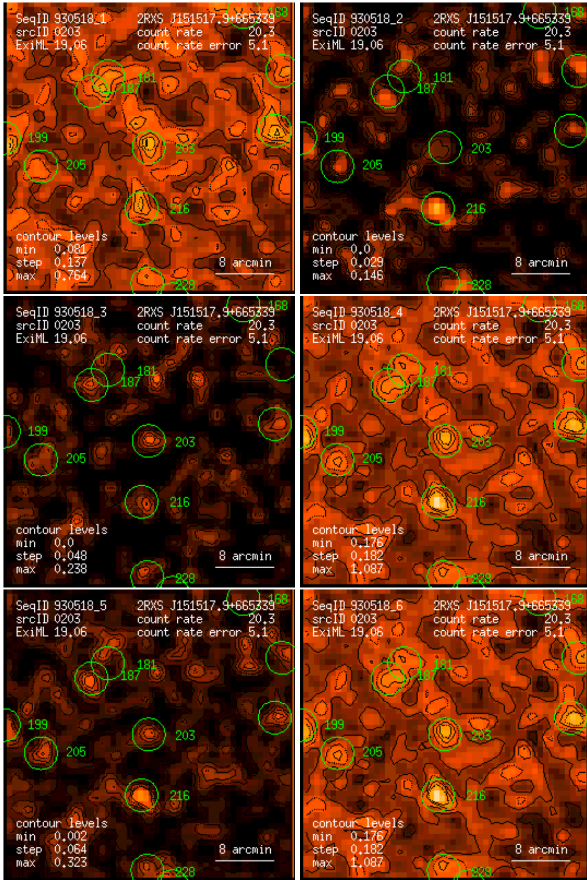
Figure 203: RASS 930518: detection 0203: band rate images, Gaussian filter: (1) PSPC channels 11 – 41, (2) 52 – 90, (3) 91 – 201, (4) 11 – 235, (5) 52 – 201, (6) 11 – 201. Broad band rates in counts/ks. Band rate contour levels in counts/ks/arcmin 2 .
