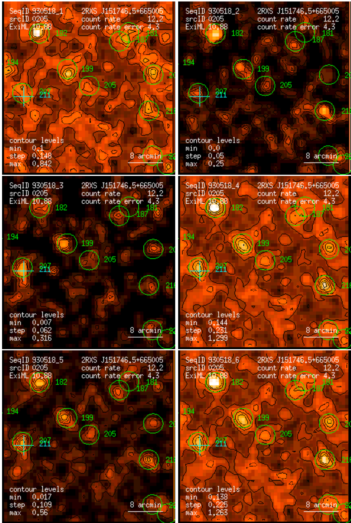
Figure 205: RASS 930518: detection 0205: band rate images, Gaussian filter: (1) PSPC channels 11 – 41, (2) 52 – 90, (3) 91 – 201, (4) 11 – 235, (5) 52 – 201, (6) 11 – 201. Broad band rates in counts/ks. Band rate contour levels in counts/ks/arcmin 2 .
