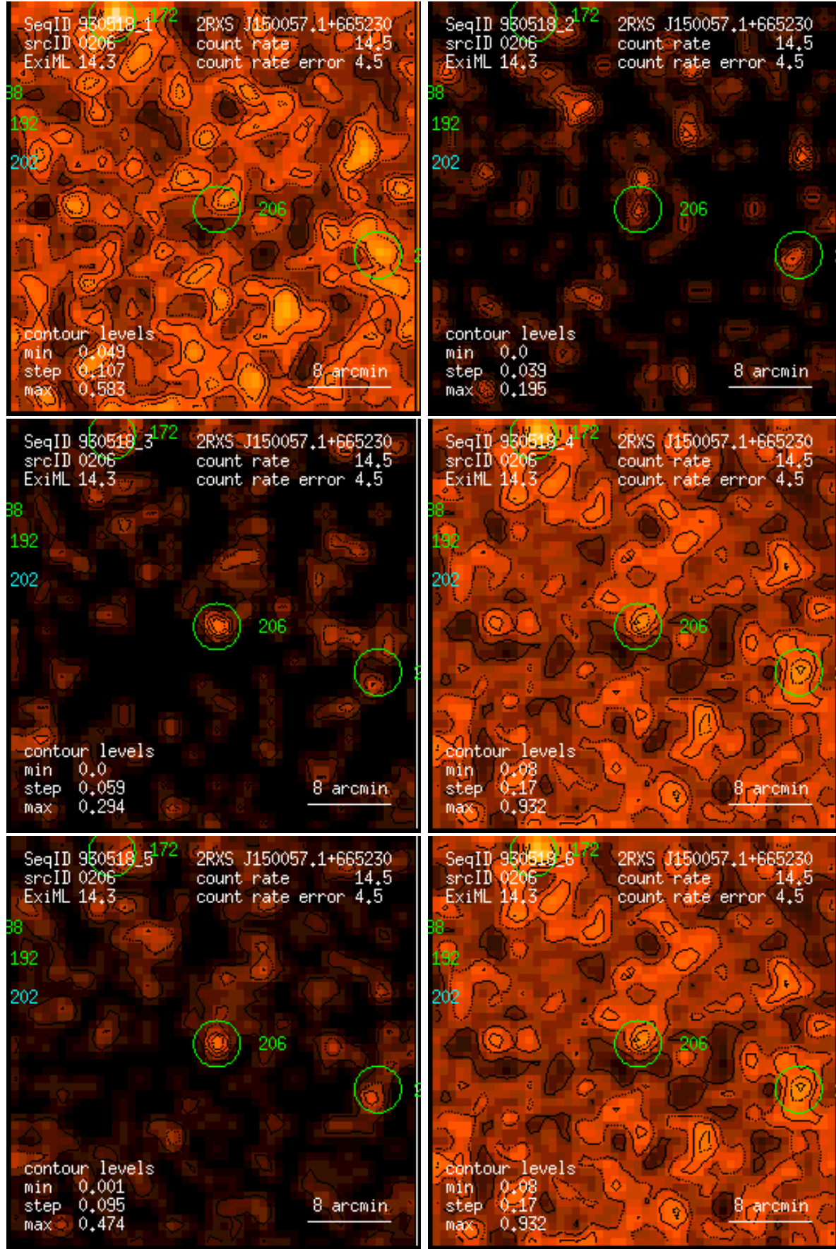
Figure 206: RASS 930518: detection 0206: band rate images, Gaussian filter: (1) PSPC channels 11 – 41, (2) 52 – 90, (3) 91 – 201, (4) 11 – 235, (5) 52 – 201, (6) 11 – 201. Broad band rates in counts/ks. Band rate contour levels in counts/ks/arcmin 2 .
